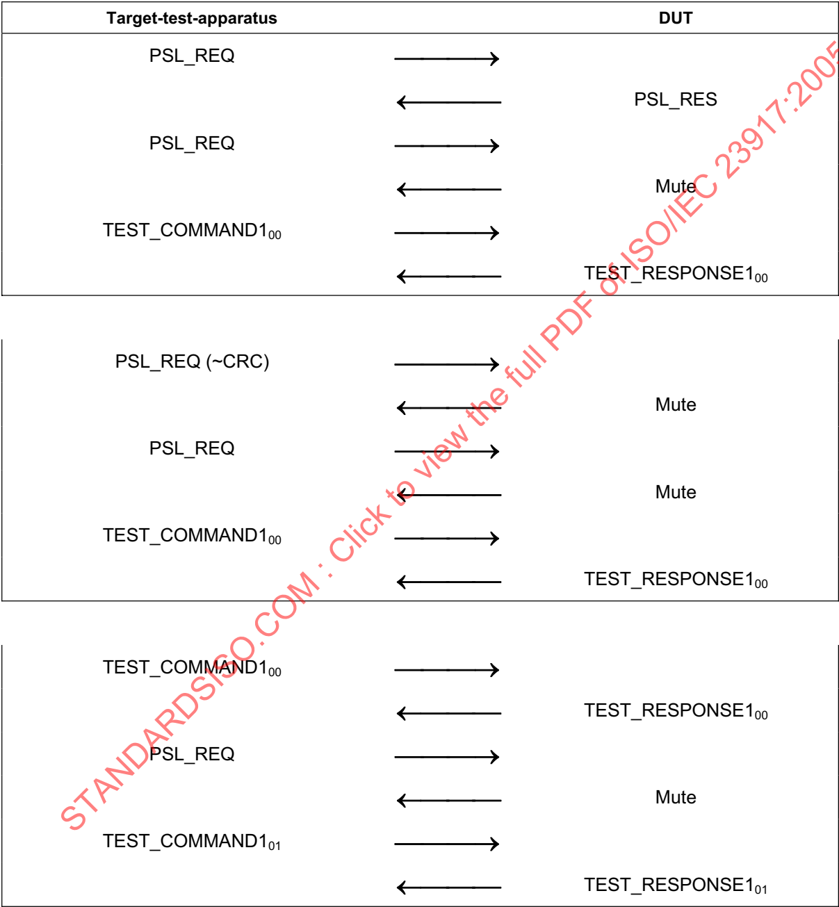
Scenario T 2 — PSL_REQ
