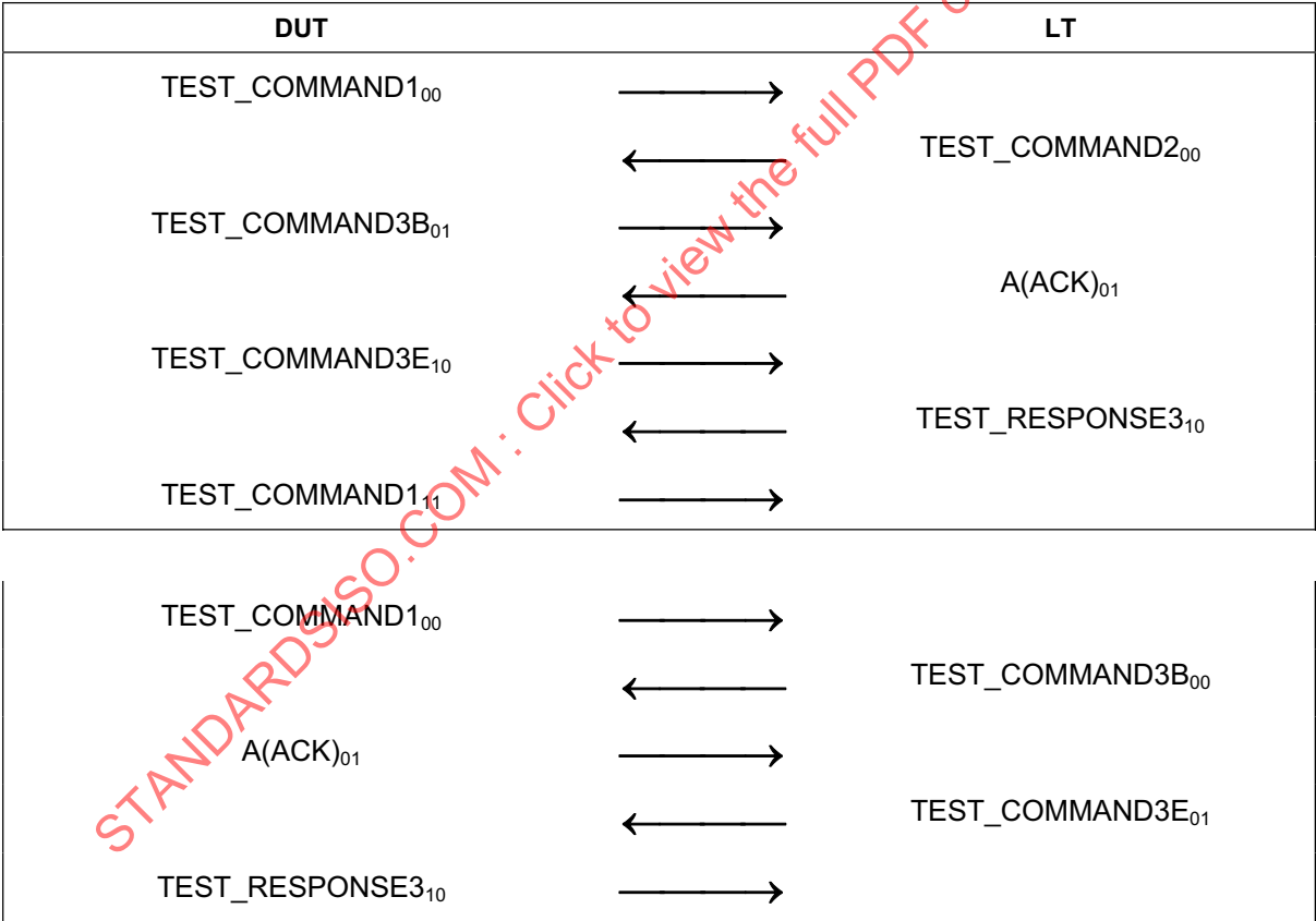
Scenario I 5 — DEP_RES with more information bit set to ONE, correct transaction
