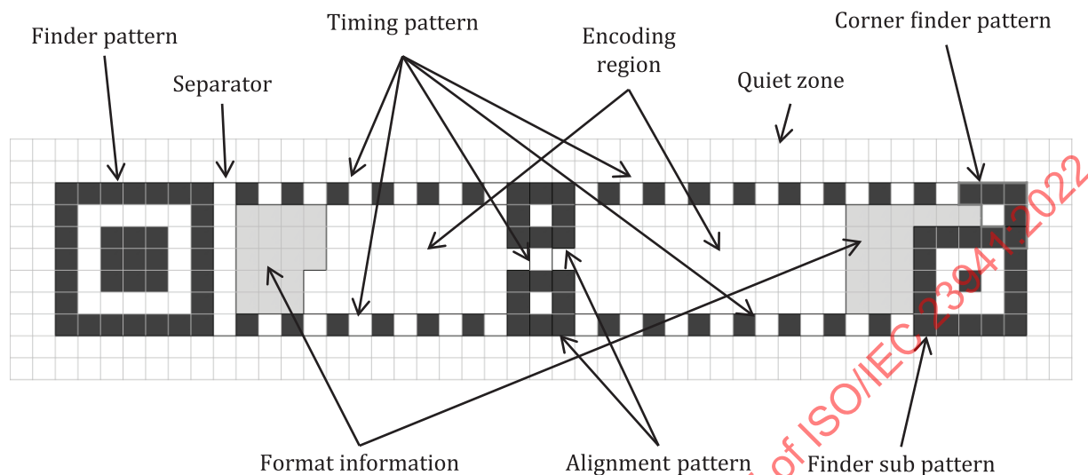
Figure 2 — Structure of Version R7x43 rMQR symbol
