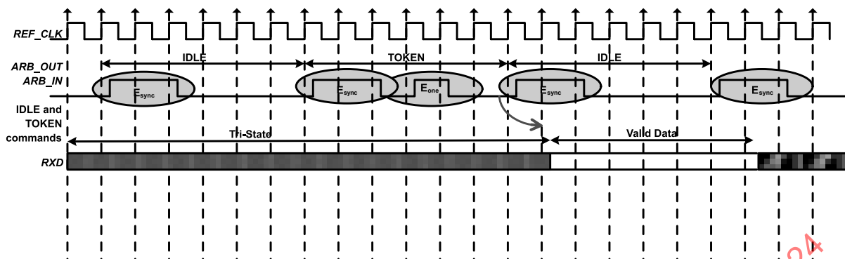
Figure 12 – Op-code to RXD relationship
