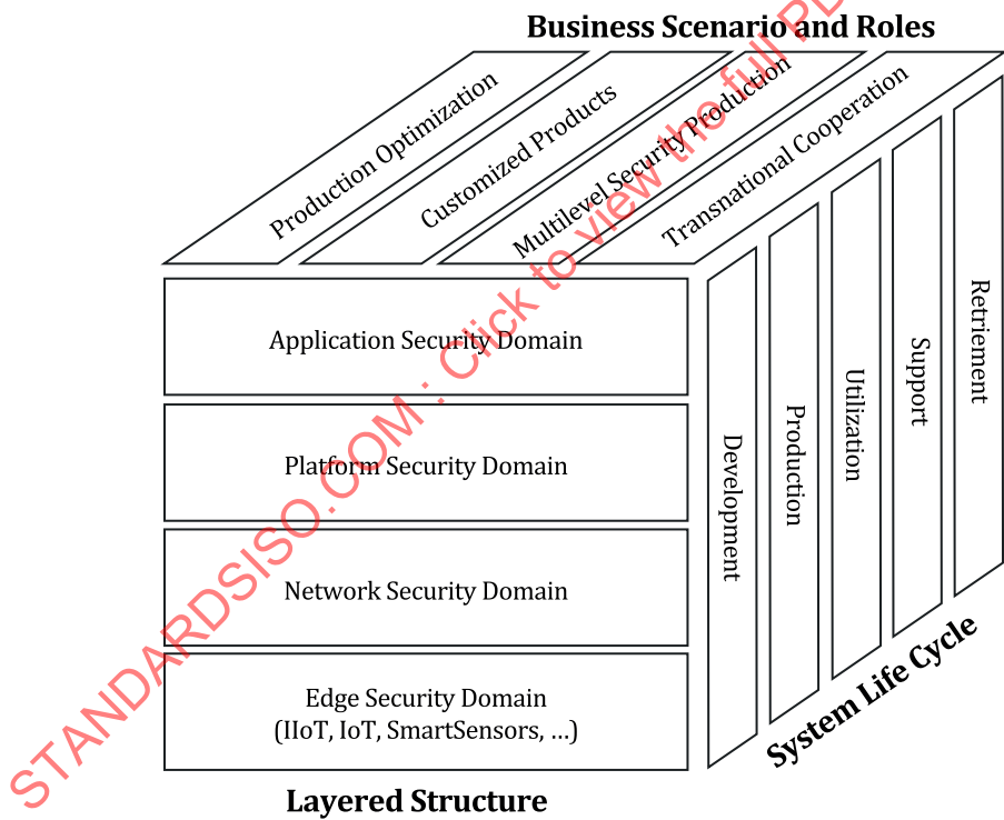
Figure 3 — Security reference model of an IIP
