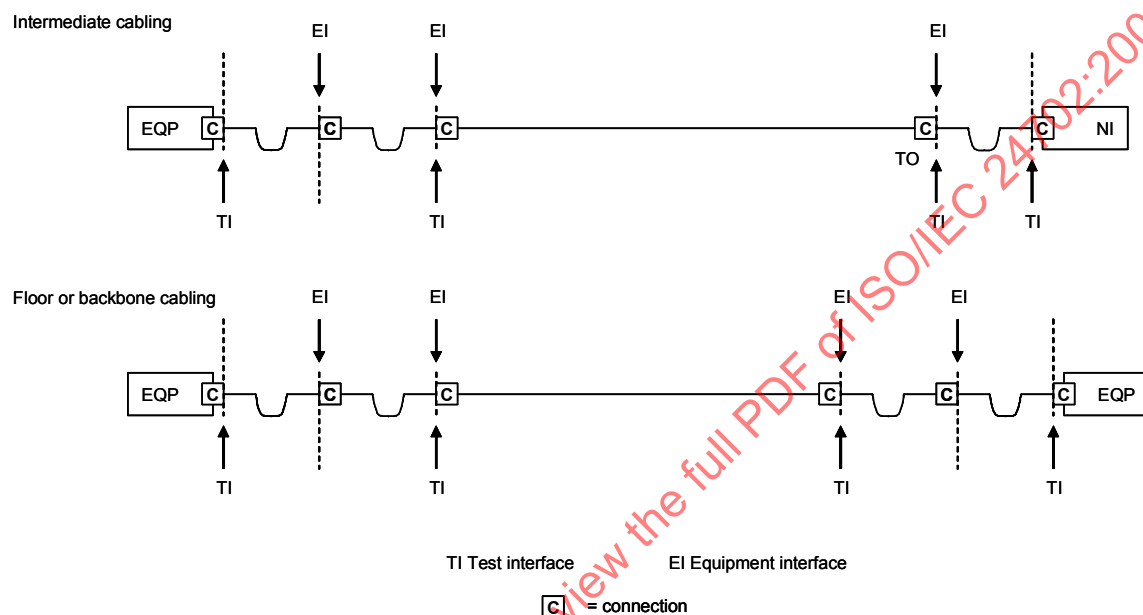
Figure 7 – Test and equipment interfaces
