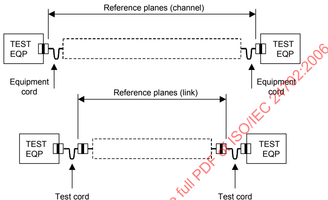
Figure B.1 – Reference planes for link and channels (point-to-point)
