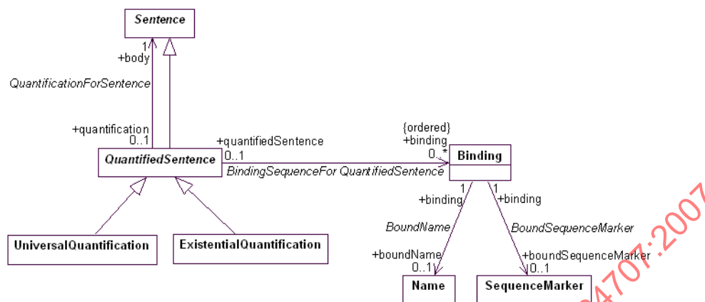
Figure 4 — Abstract syntax of a quantified sentence
