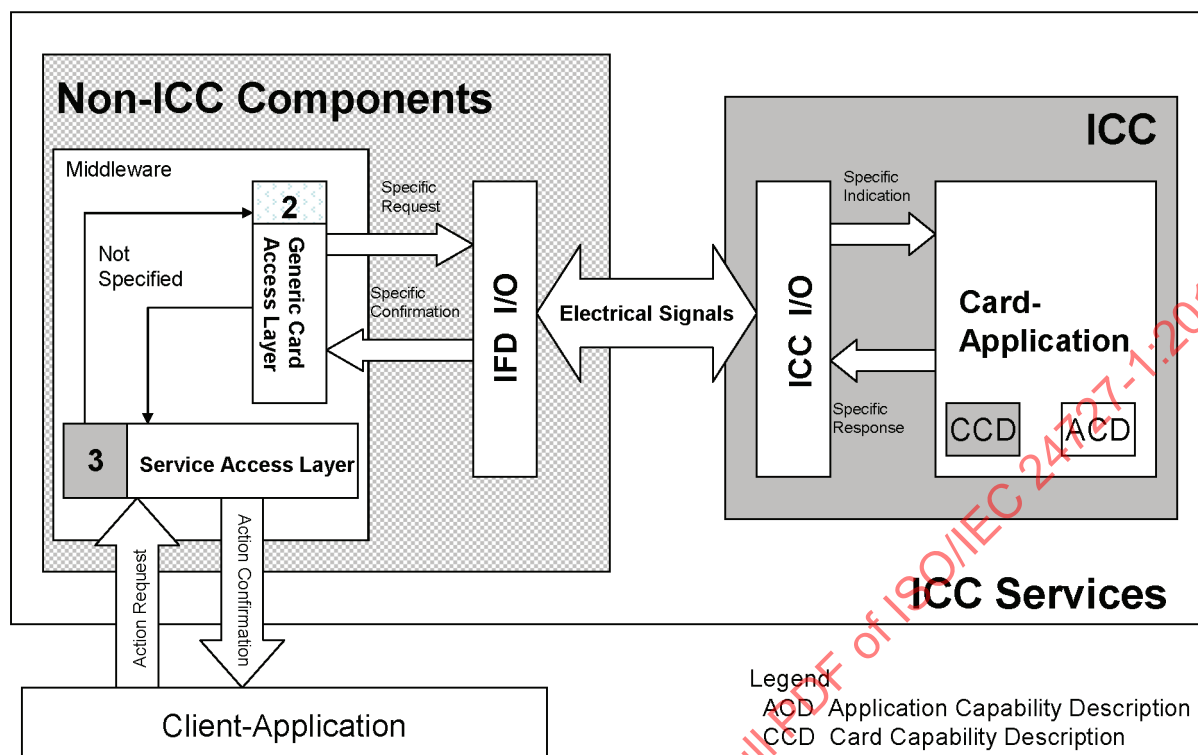
Figure A.3 — Combined implementation
