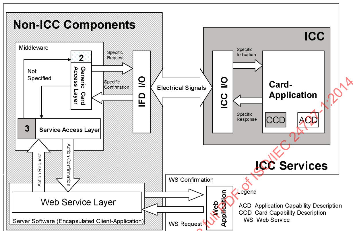
Figure A.7 — Web service configuration
