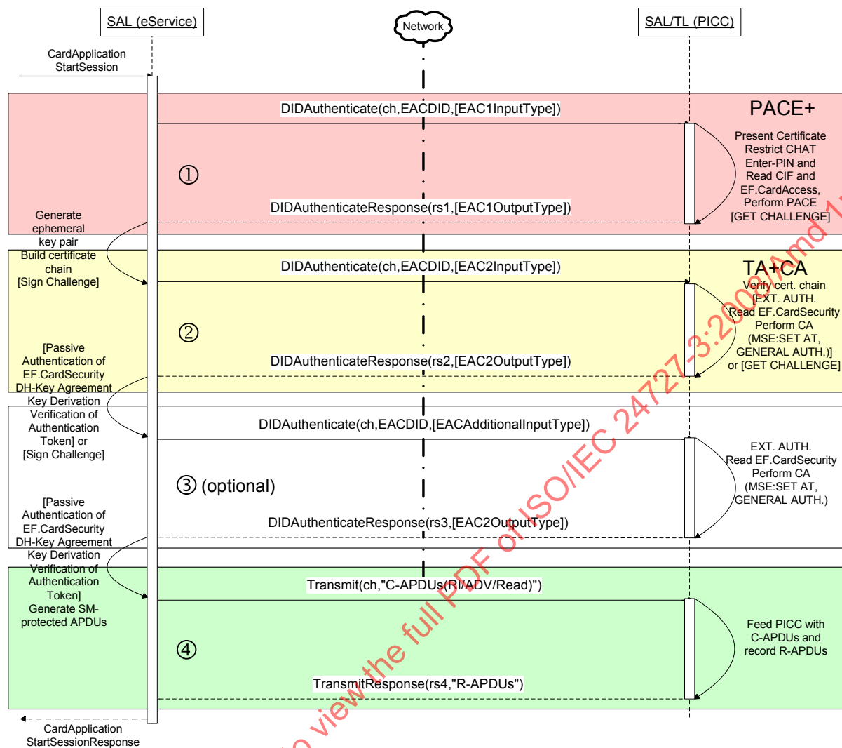
Figure E.1: Message sequence between SAL's after CardApplicationStartSession (M-EAC)
