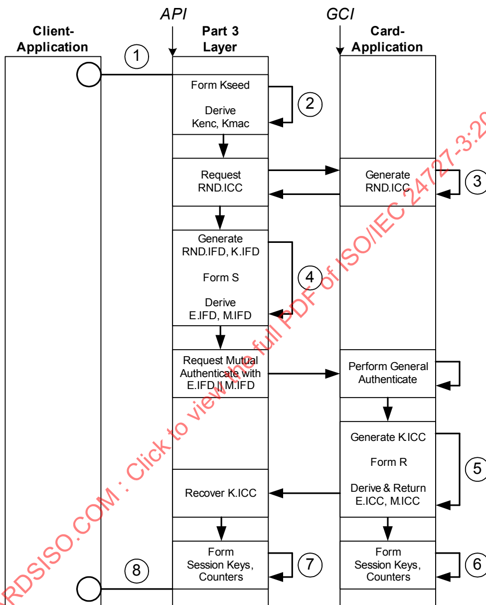
Figure A.9 — Mutual Authentication with Key Establishment
