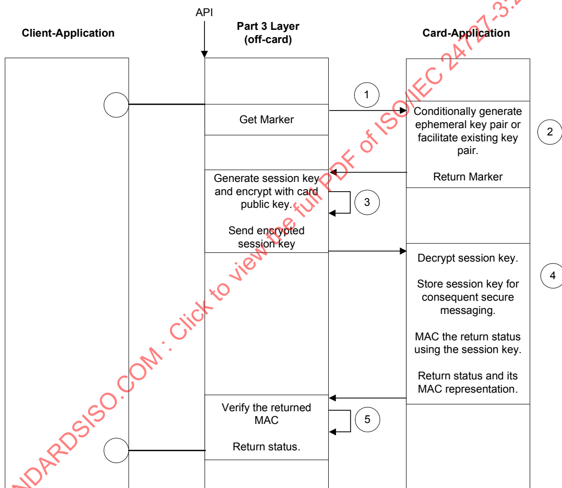
Figure A.15 — Asymmetric Session Key Establishment
