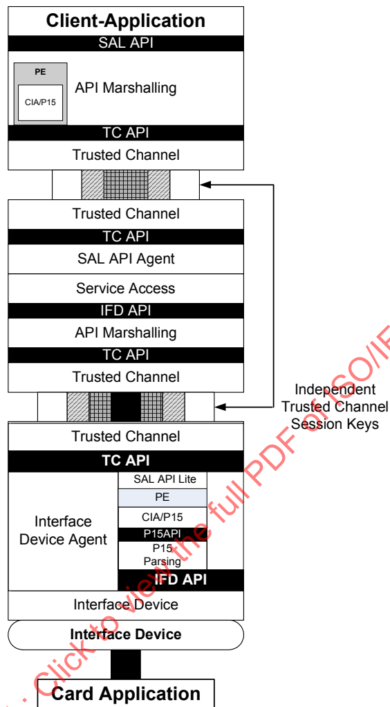
Figure D4 – Proposed Full Network Stack
