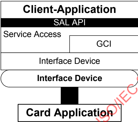
Figure D5 – Current Loyal Stack
