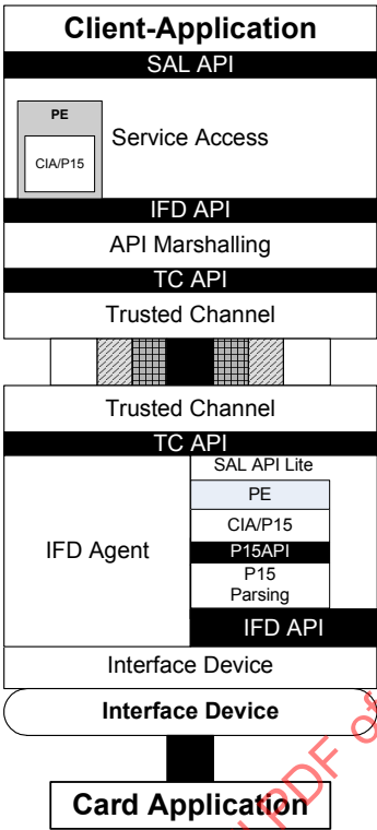
Figure D8 – Proposed Opaque-ICC Stack
