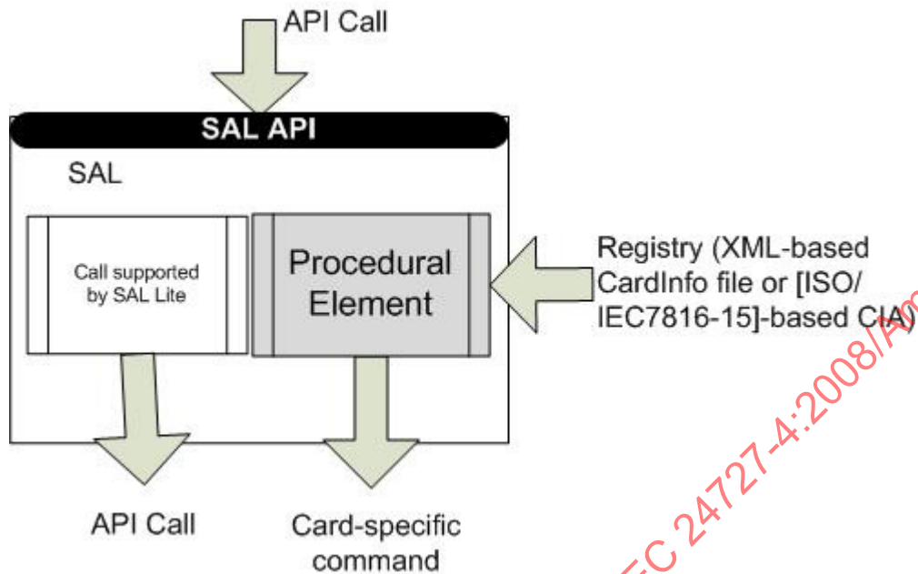
Figure D1 – Procedural Element functionality
