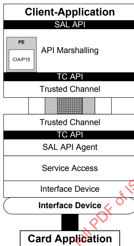
Figure D10 – Proposed Remote-loyal Stack
