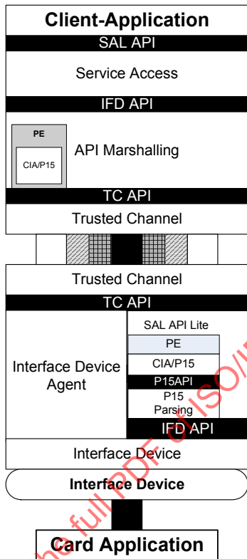
Figure D12 – Proposed Remote-ICC Stack
