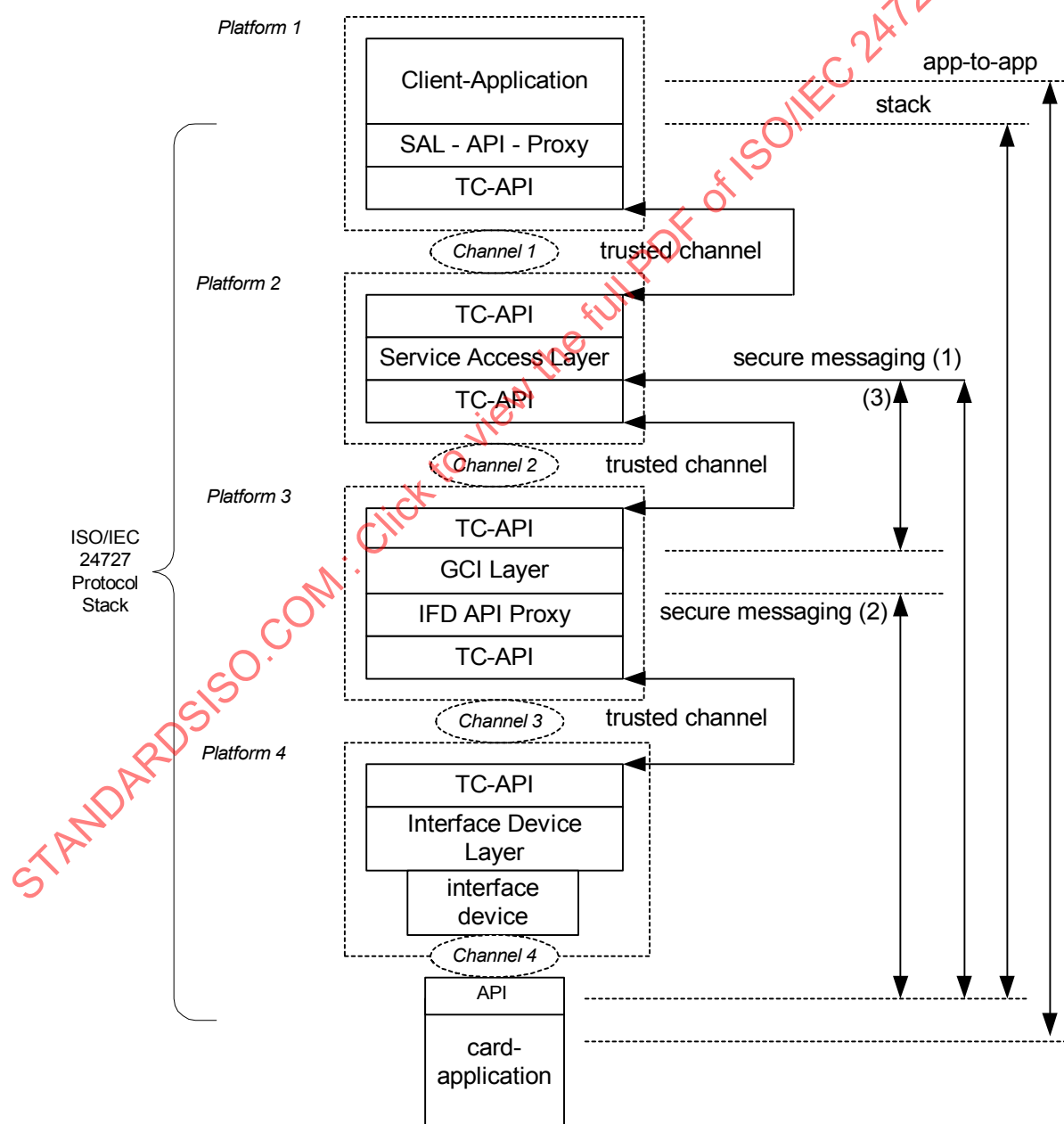
Figure 2 — Generic Elements of the ISO/IEC 24727 Stack
