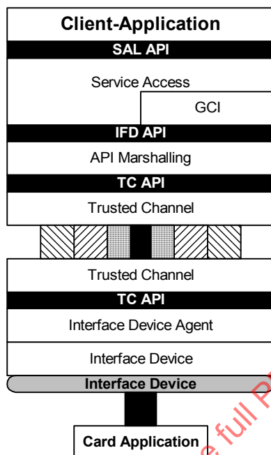
Stack Configuration
