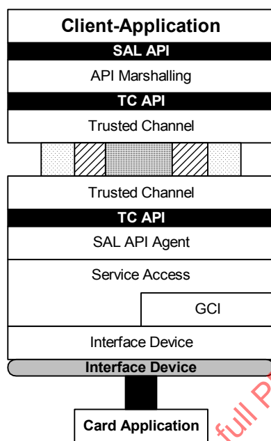
Stack Configuration
