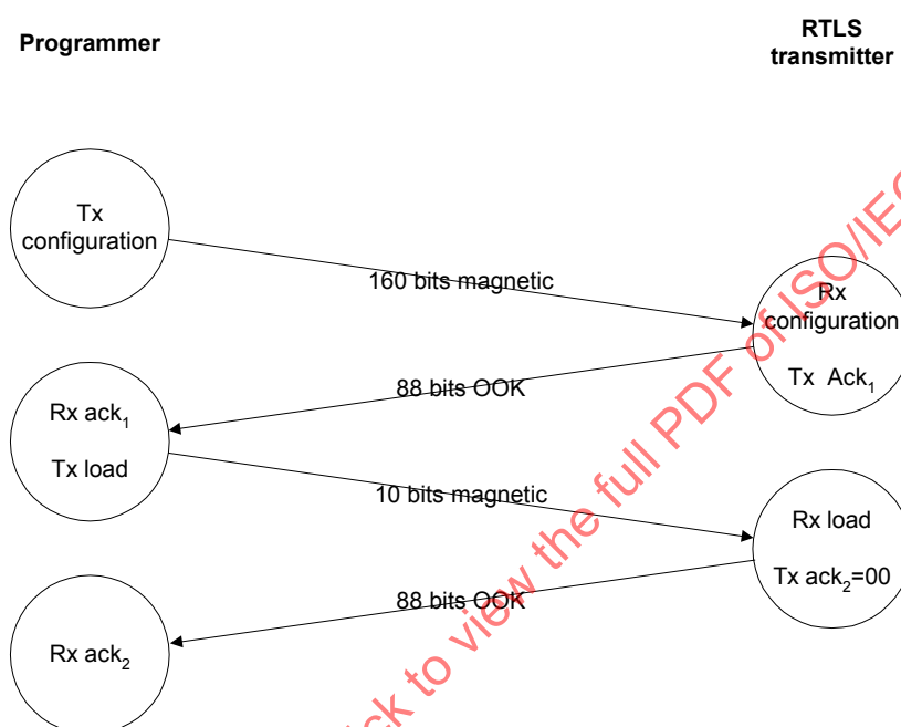
Figure 8 — Write configuration message exchange
