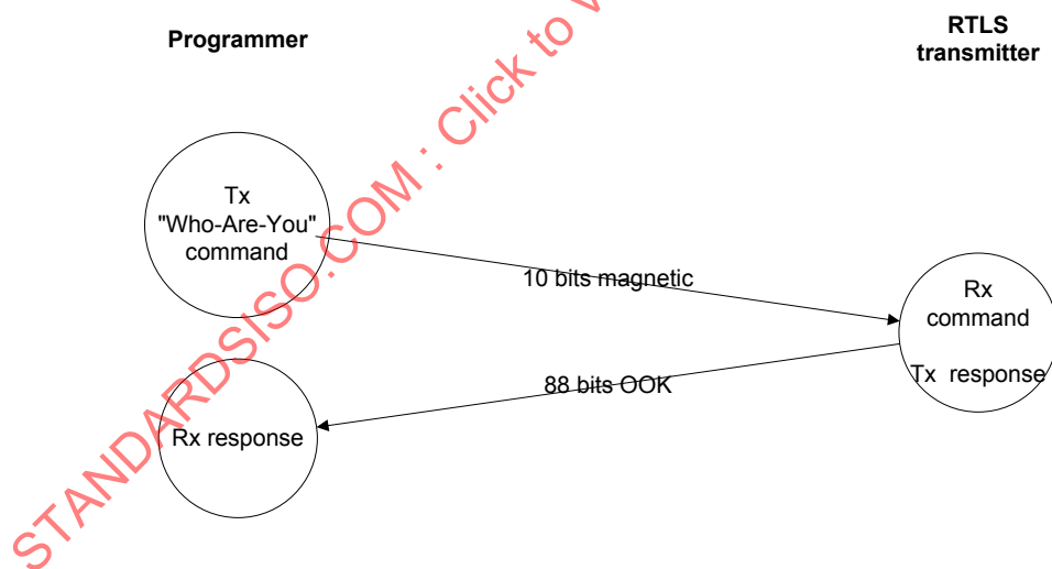
Figure 14 — Who-Are-You command protocol
