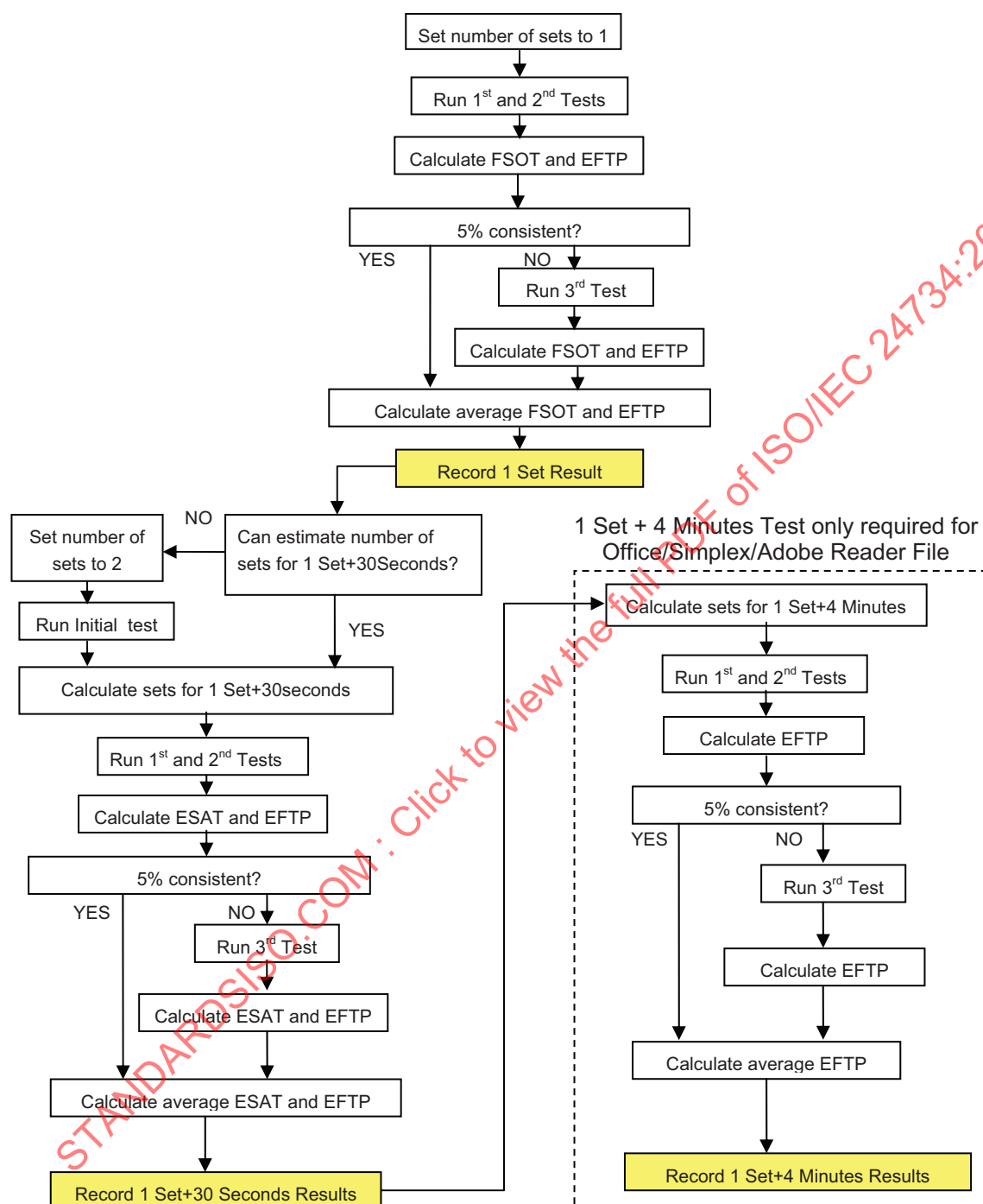
Figure 1 — Test Method Process Flow Chart
