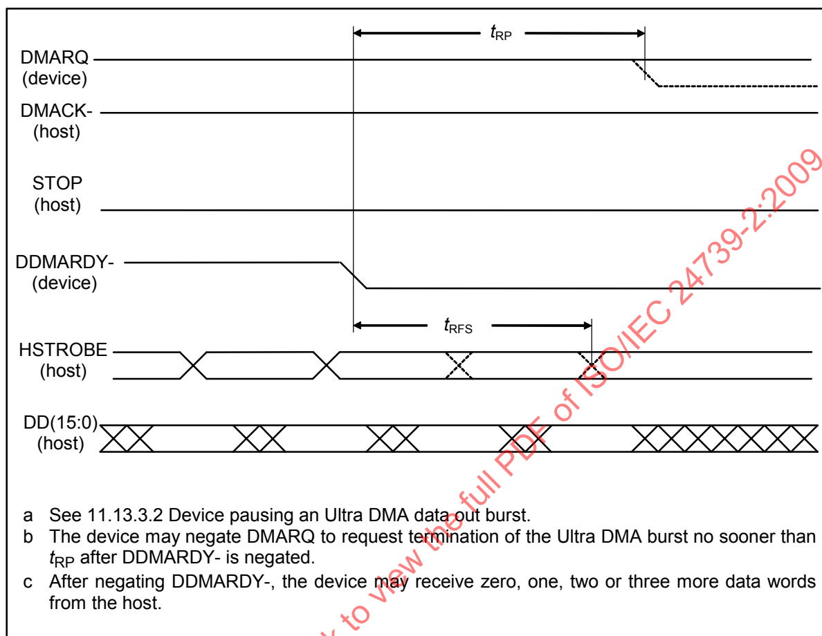
Figure 78 – Device pausing an Ultra DMA data-out burst
