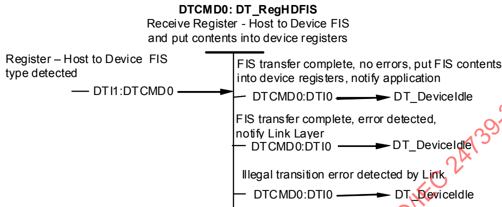
Figure 89 – Device transport decompose register – Host to Device state diagram (State DTCMD0)
