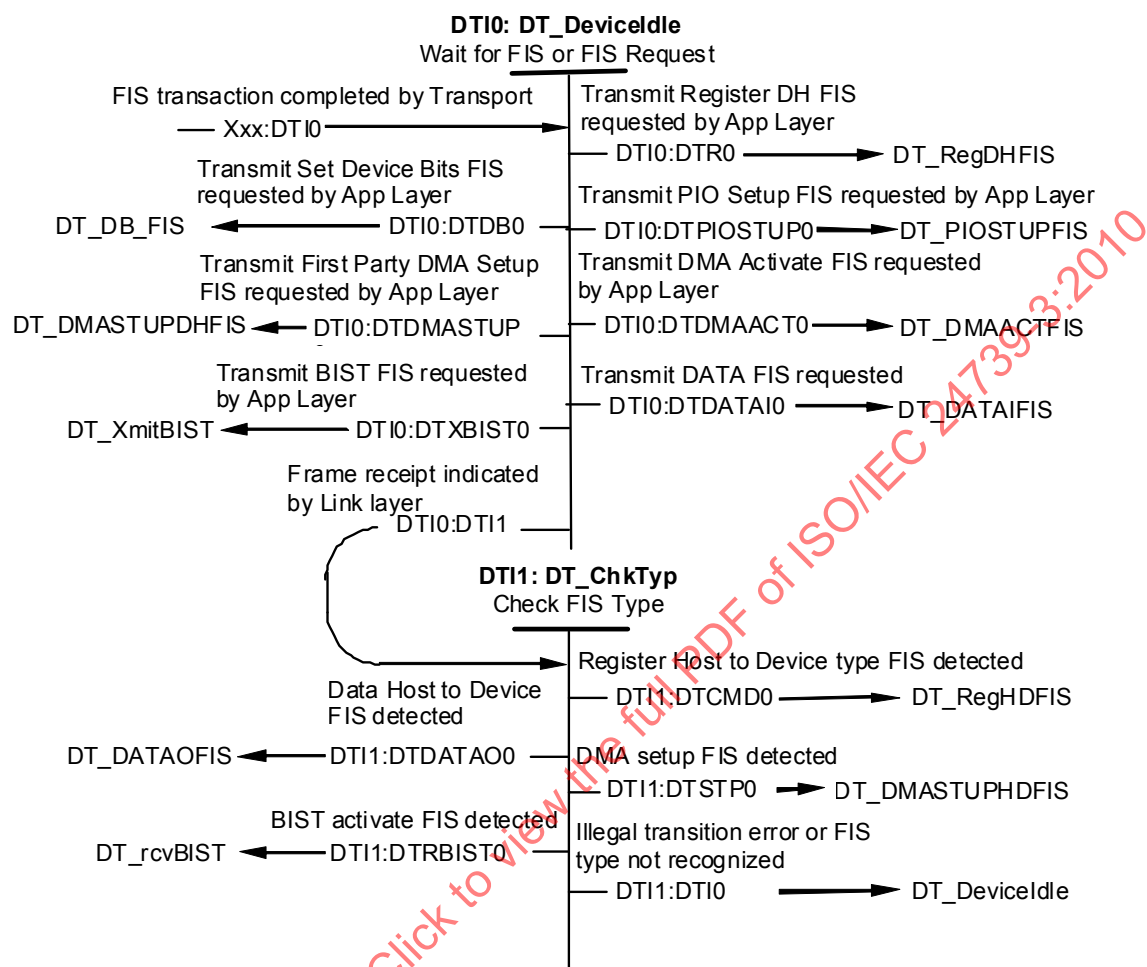
Figure 81 – Device transport idle state diagram (States DTI0-DTI1)
