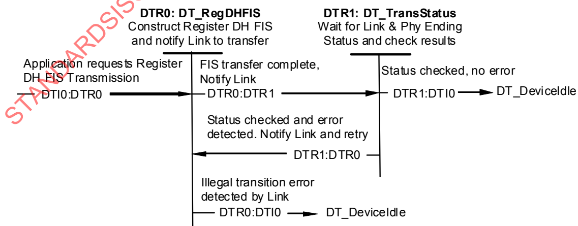
Figure 82 – Device transport send register – Device to host state diagram (DTR0-DTR1)
