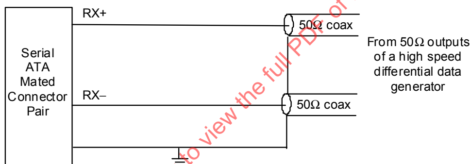
Figure 32 – Receive test fixture
