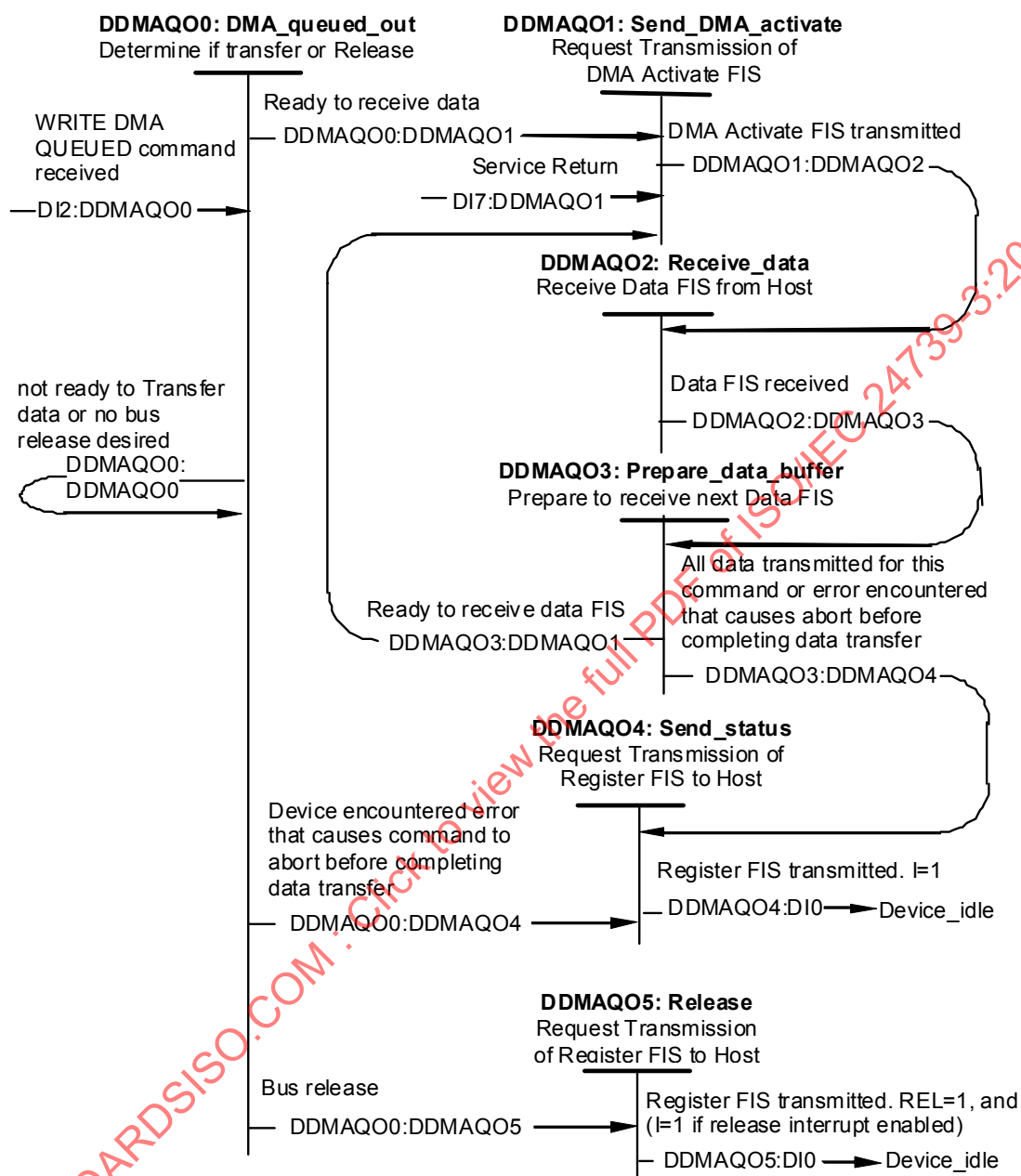
Figure 105 – WRITE DMA QUEUED command protocol (DDMAOQ0-DDMAQO5)
