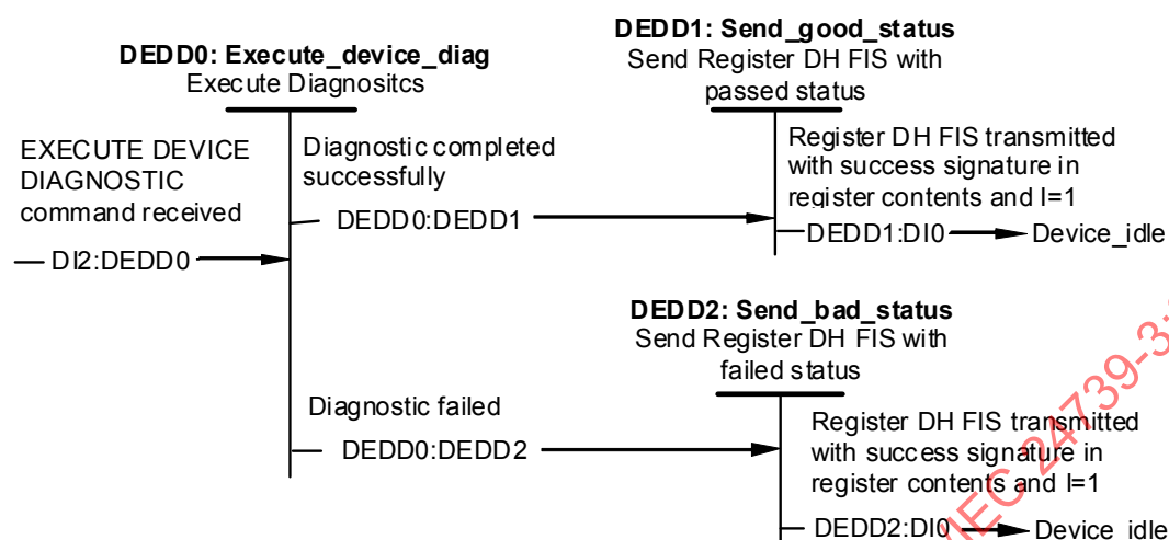
Figure 96 – EXECUTE DEVICE DIAGNOSTIC command protocol (States DEDD0-DEDD2)
