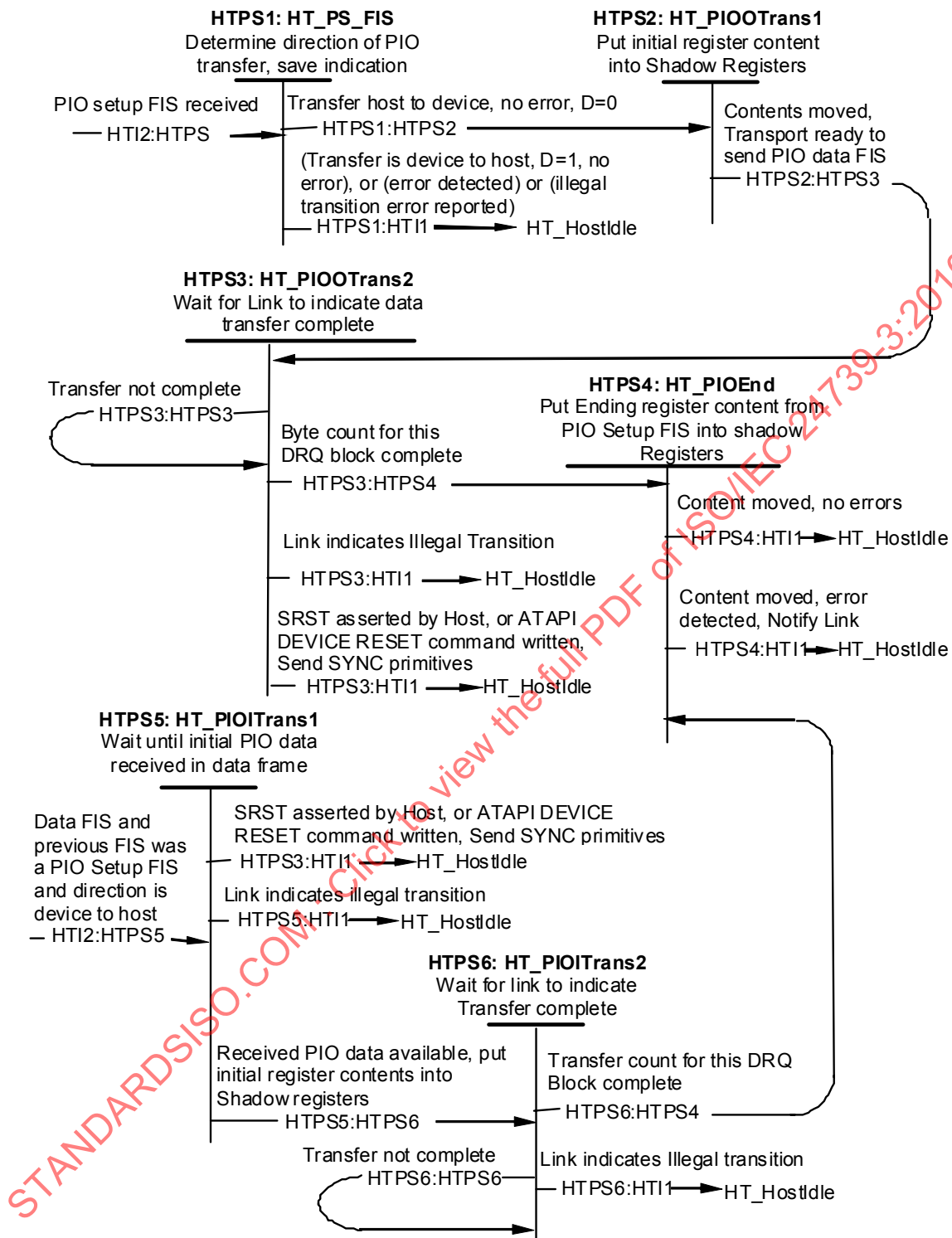
Figure 78 – Host transport decompose PIO setup FIS state diagram (States HTPS1- HTPS6)
