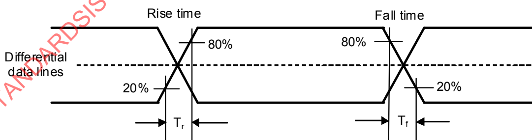
Figure 30 – Signal rise and fall times
