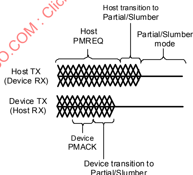
Figure 44 – ON to Partial/Slumber, host initiated
