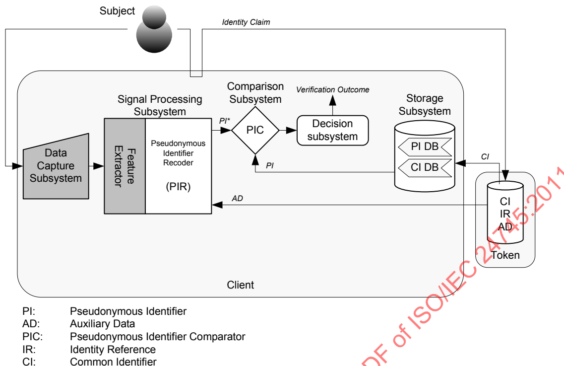
Figure 19 — Model H: Store distributed on token and client, compare on client
