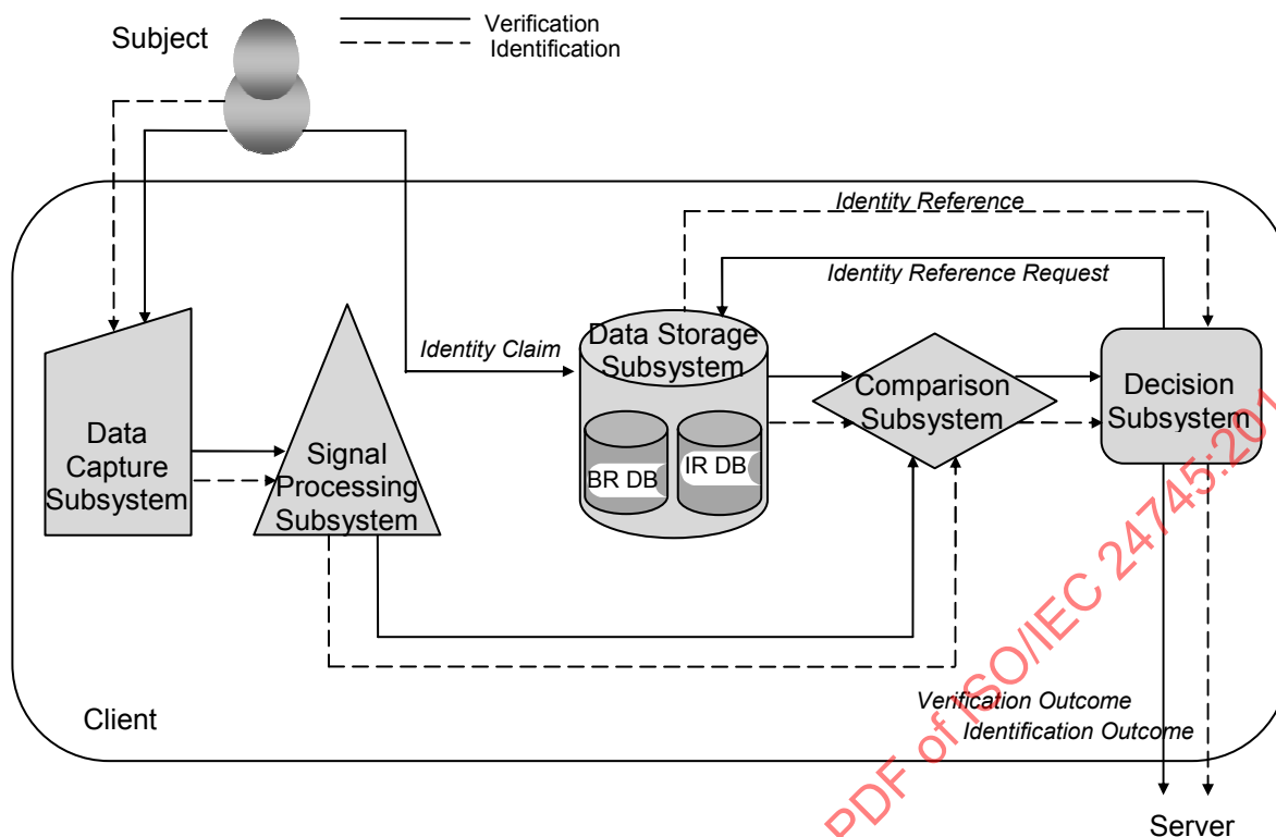
Figure 12 — Model D: Store on client and compare on client using BRs
