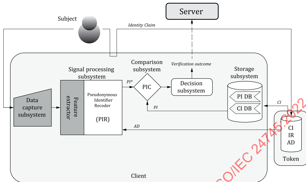
Figure 20 — Model H: Store distributed on token and client, compare on client
