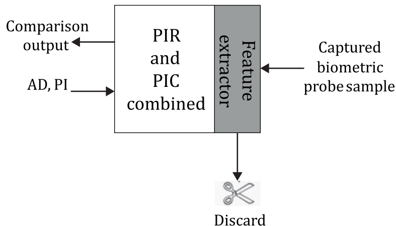
Figure B.3 — Signal processing and comparison combined
