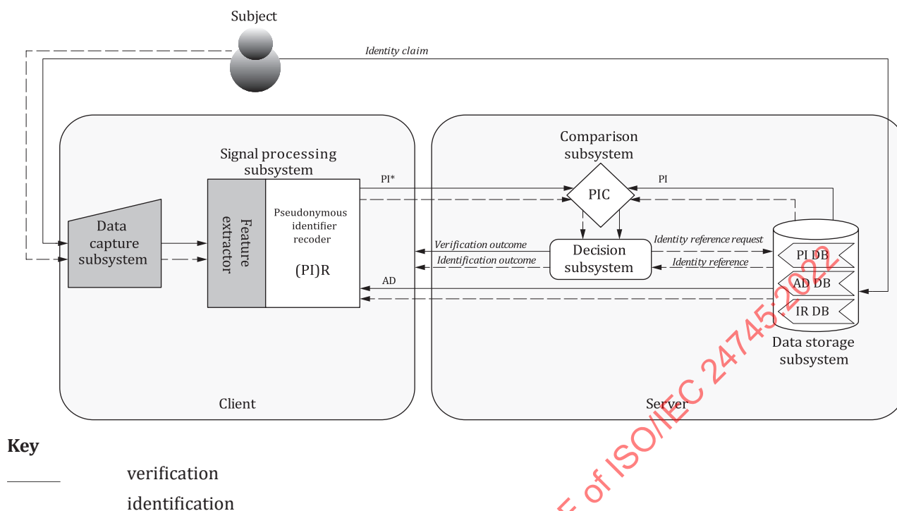
Figure 8 — Model A: Store on server and compare on server using RBRs
