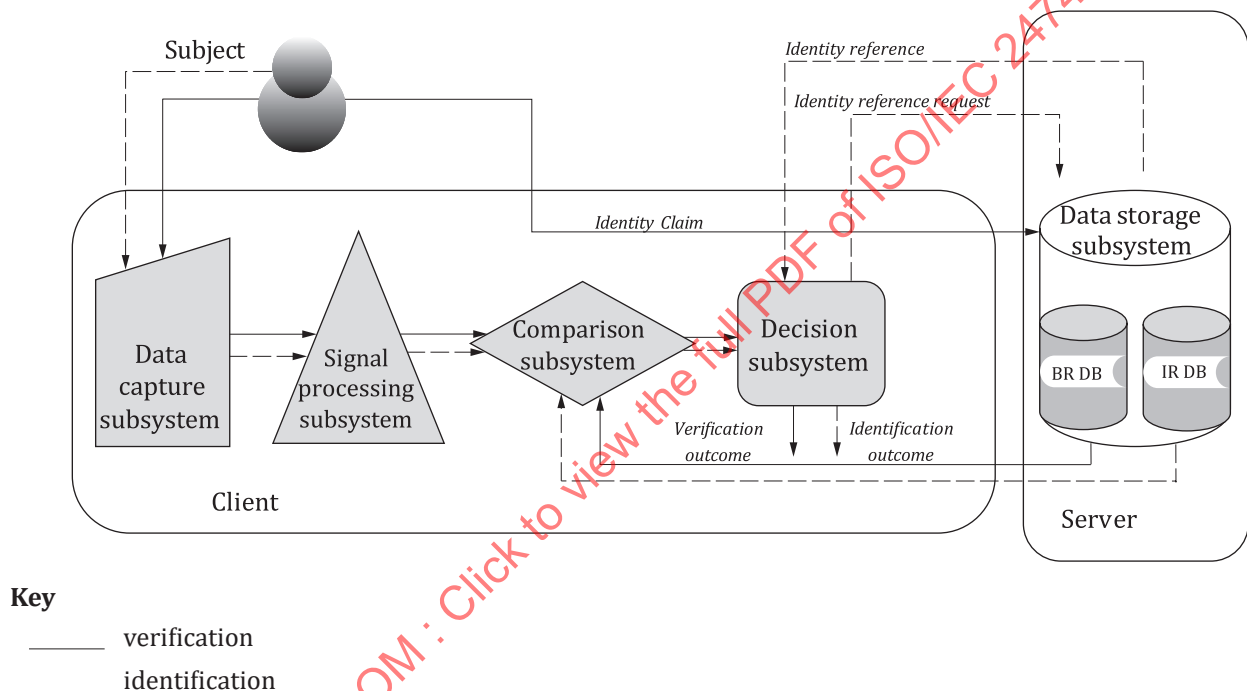
Figure 11 — Model C: Store on server and compare on client using BRs
