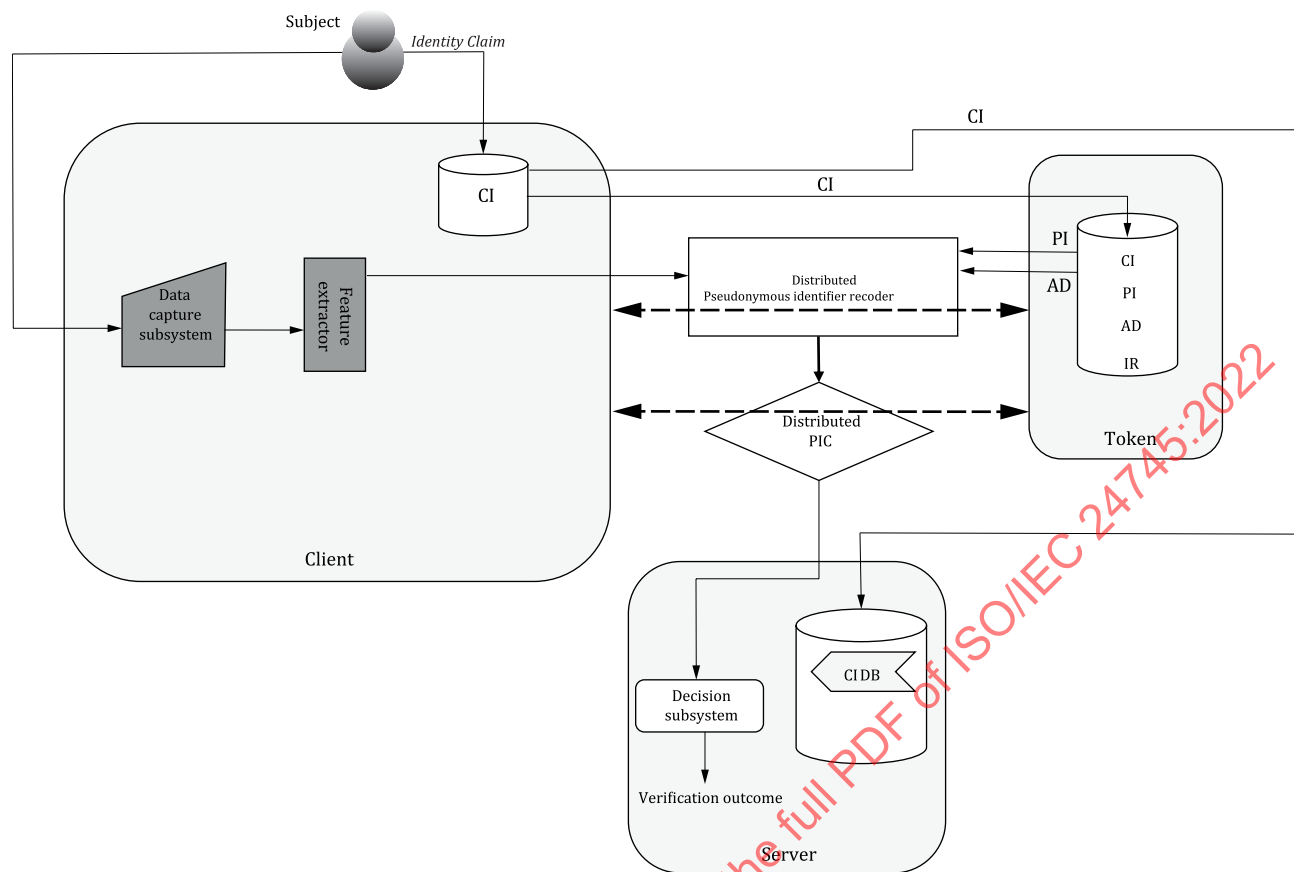
Figure 23 — Model J: Store on token, compare distributed using RBRs (variant with decision available only on server)
