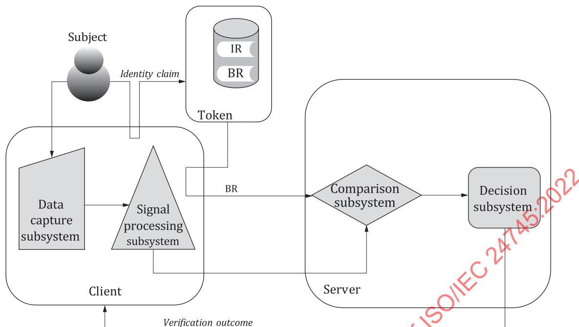
Figure 9 — Model B: Store on token and compare on server using BRs
