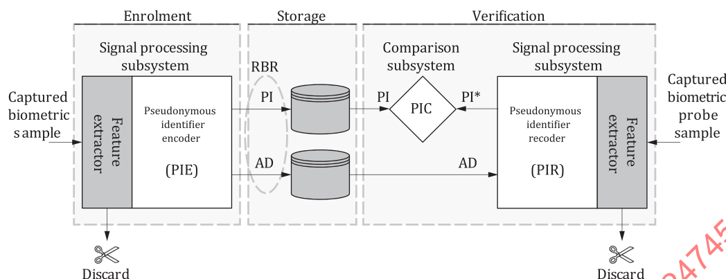
Figure 5 — Architecture for renewable biometric references (RBRs)
