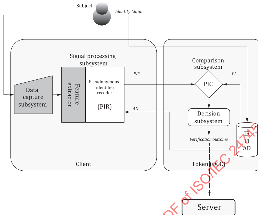
Figure 18 — Model F: Store on token and compare on token using RBRs
