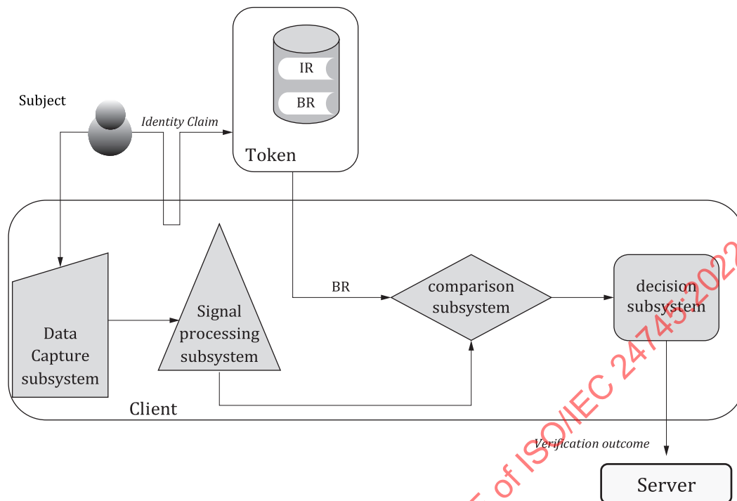
Figure 15 — Model E: Store on token and compare on client using BRs
