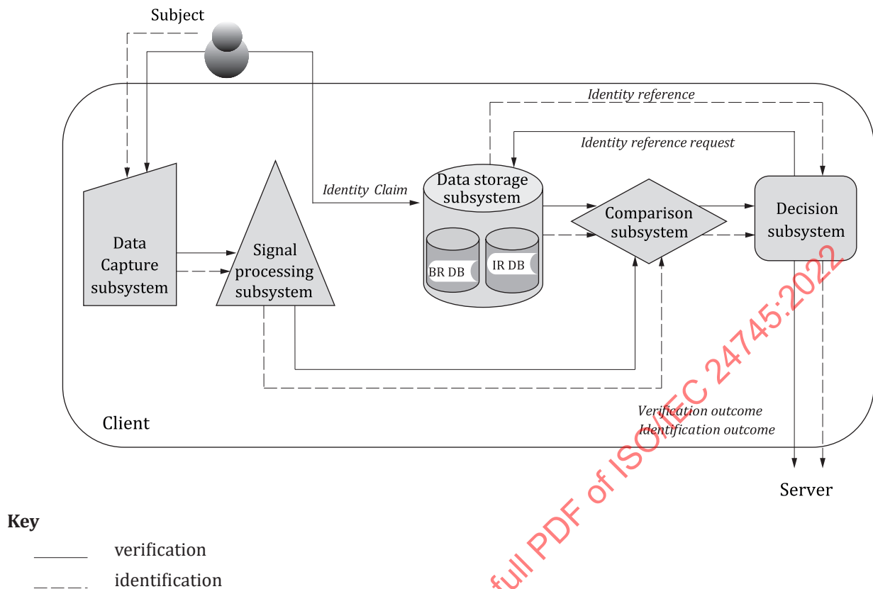
Figure 13 — Model D: Store on client and compare on client using BRs
