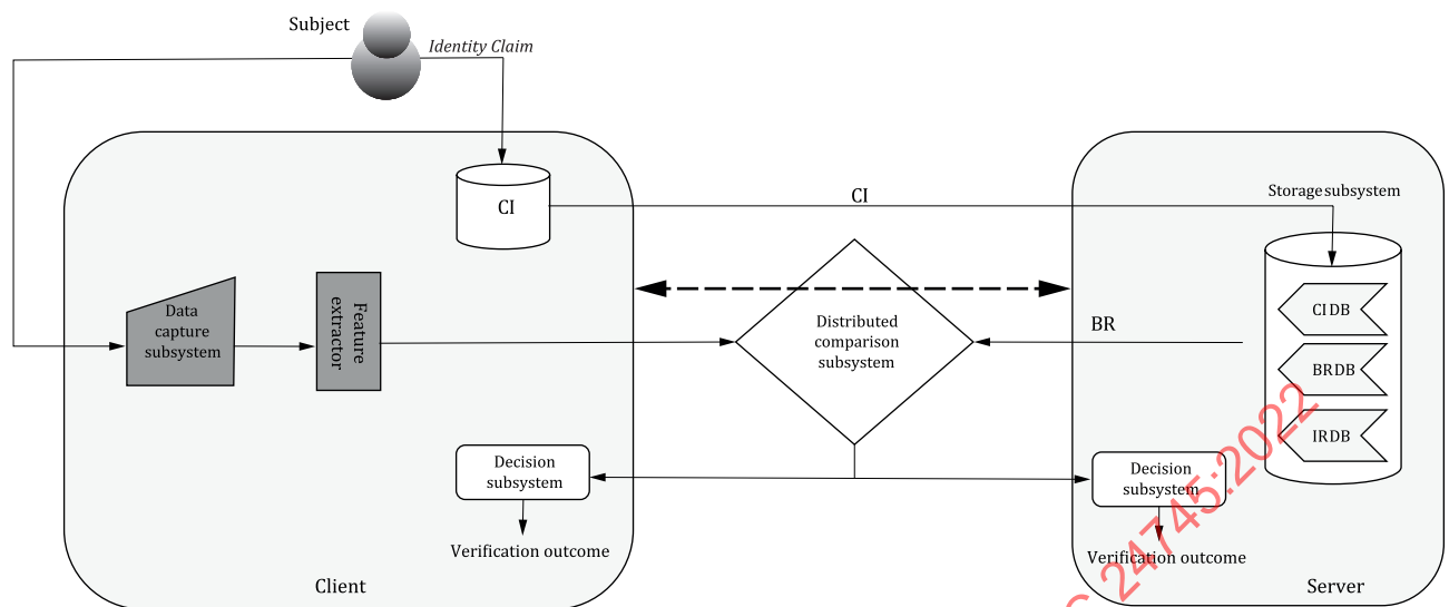
Figure 22 — Model I: Store on server, compare distributed using BRs
