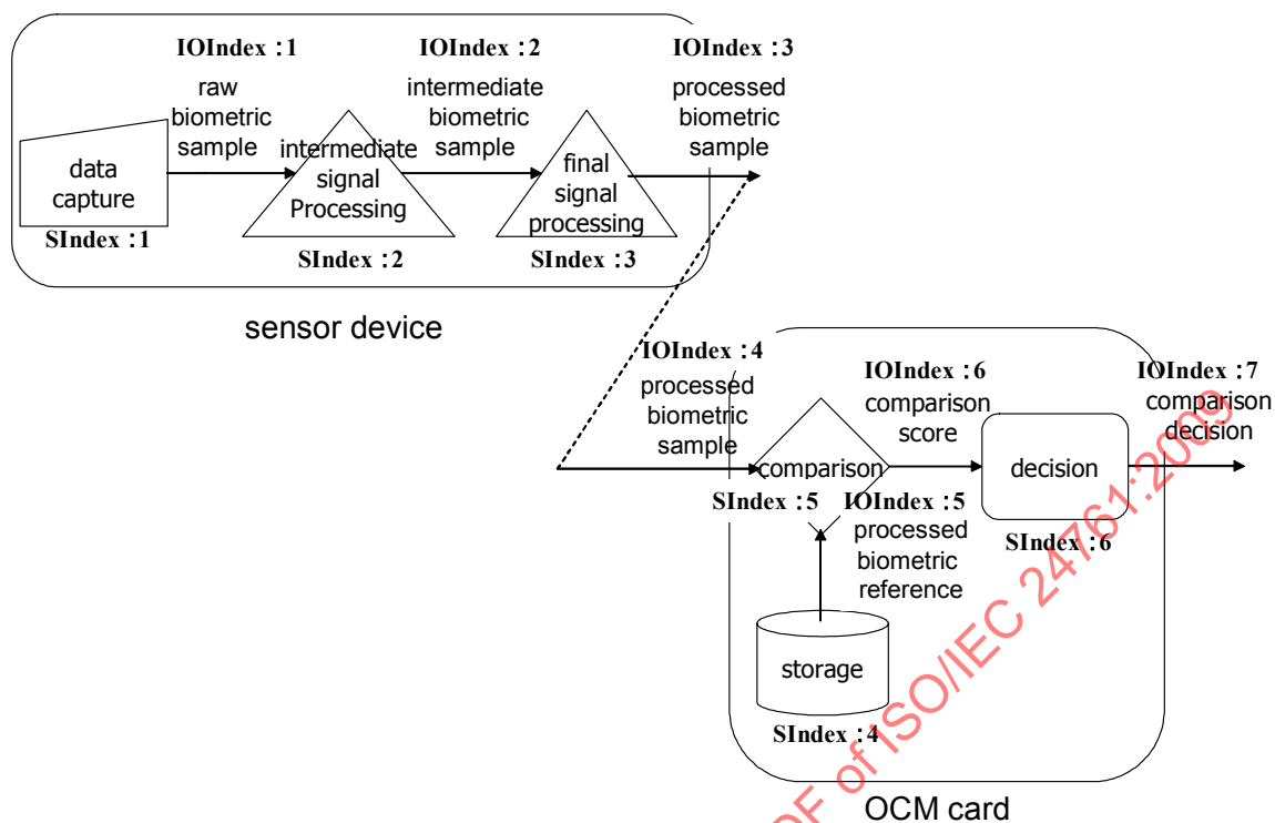
Figure B.8 — A biometric verification process of an OCM model and an example of indexing
