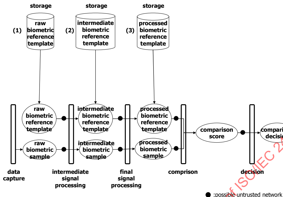
Figure 2 — Biometric verification process model
