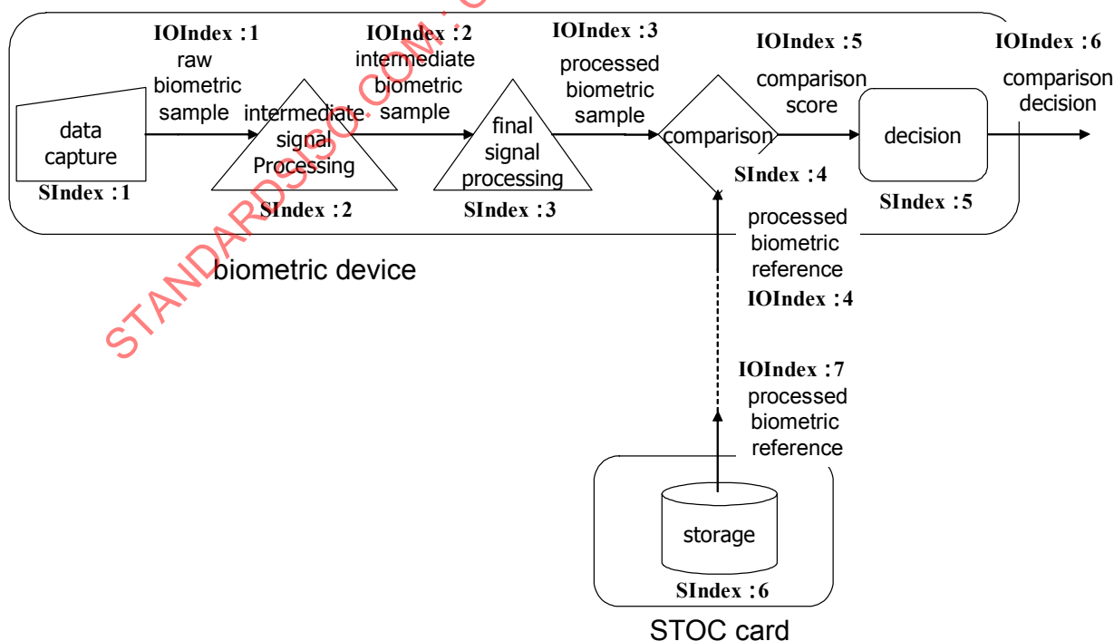
Figure B.1 — A biometric verification process of a STOC model and an example of indexing
