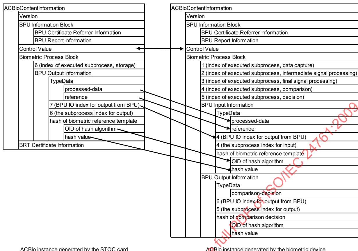
Figure B.7 — Validation of biometric verification using ACBio
