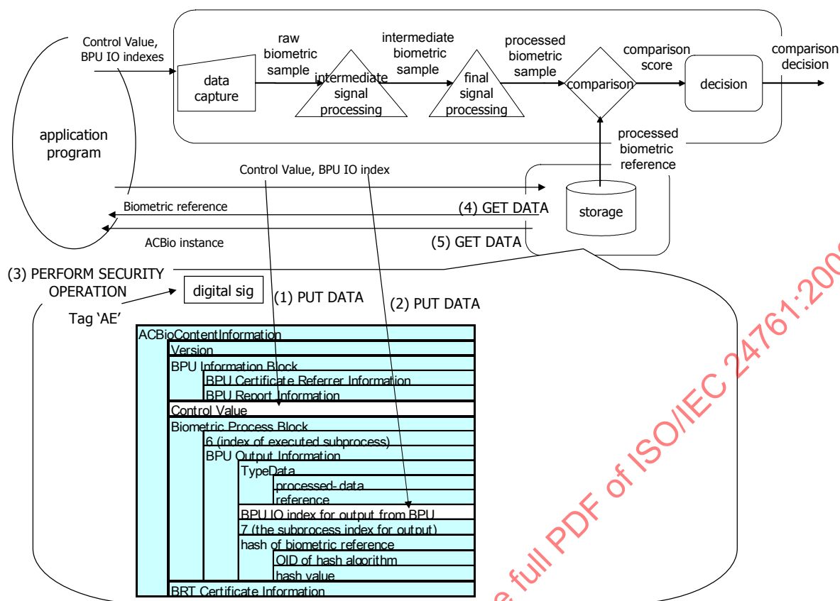
Figure B.4 — ACBio instance generation on a STOC card on an execution of a biometric verification
