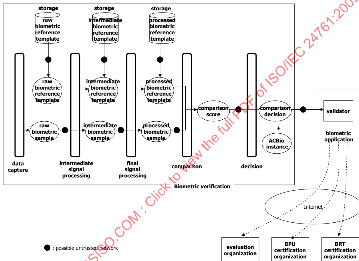
Figure 4 — Biometric verification process and its validation
