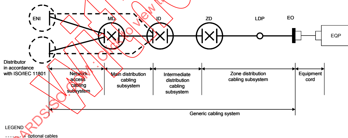
Figure C.1 – Structure of generic cabling within a data centre
