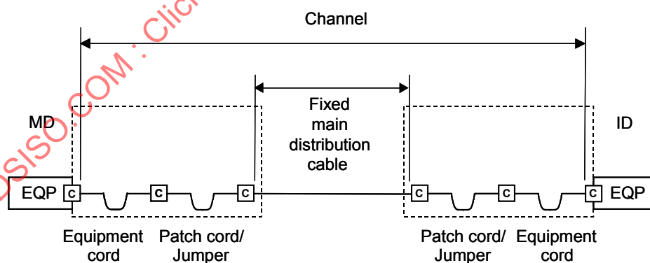
Figure C.4 – Main distribution cabling models
