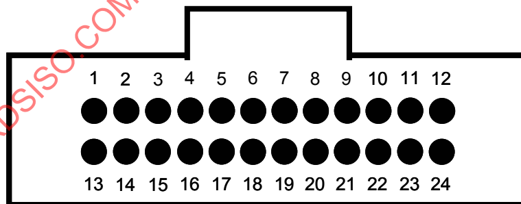
Figure 14c – IEC 61754-7 interface for 13 to 24 optical fibres
