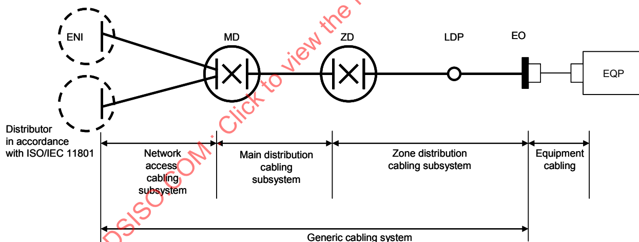
Figure 2 – Structure of generic cabling within a data centre
