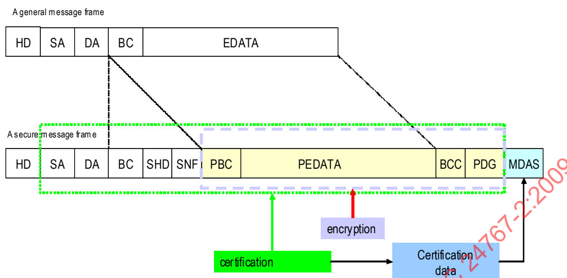
Figure 2 – General message frame versus secure message frame
