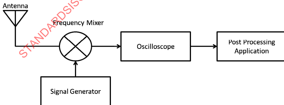
Figure 2 — Receiving setup
