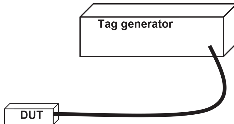
Figure 2 — Setup of equipment for UWB receiver RF Test
