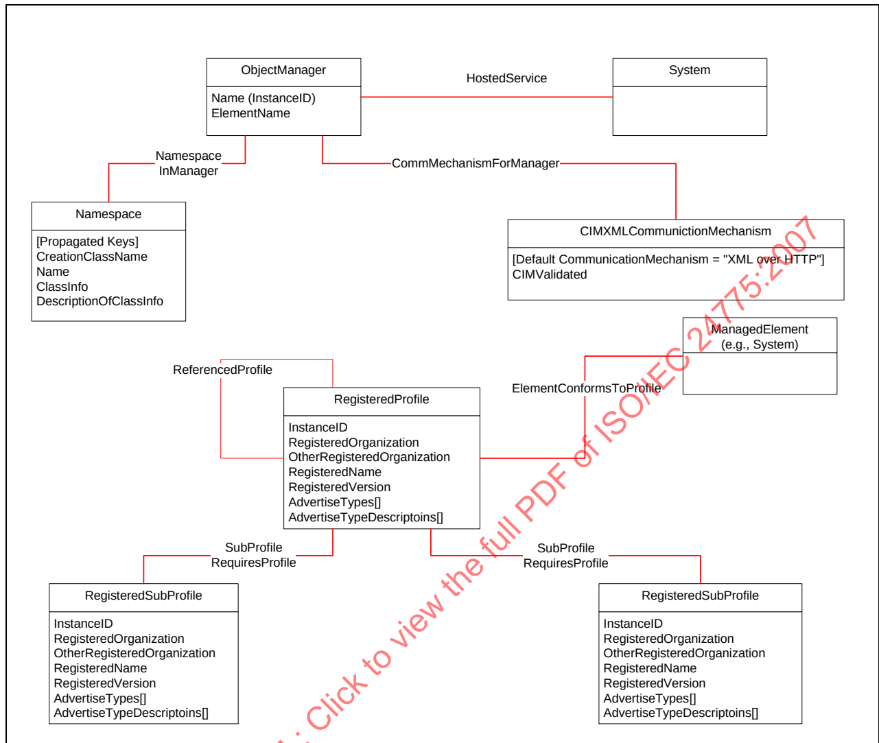
Figure 68 - Server Model
