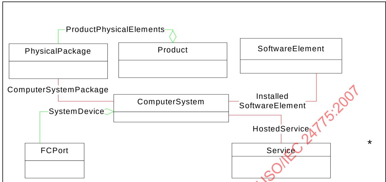
Figure 12 - Common elements
