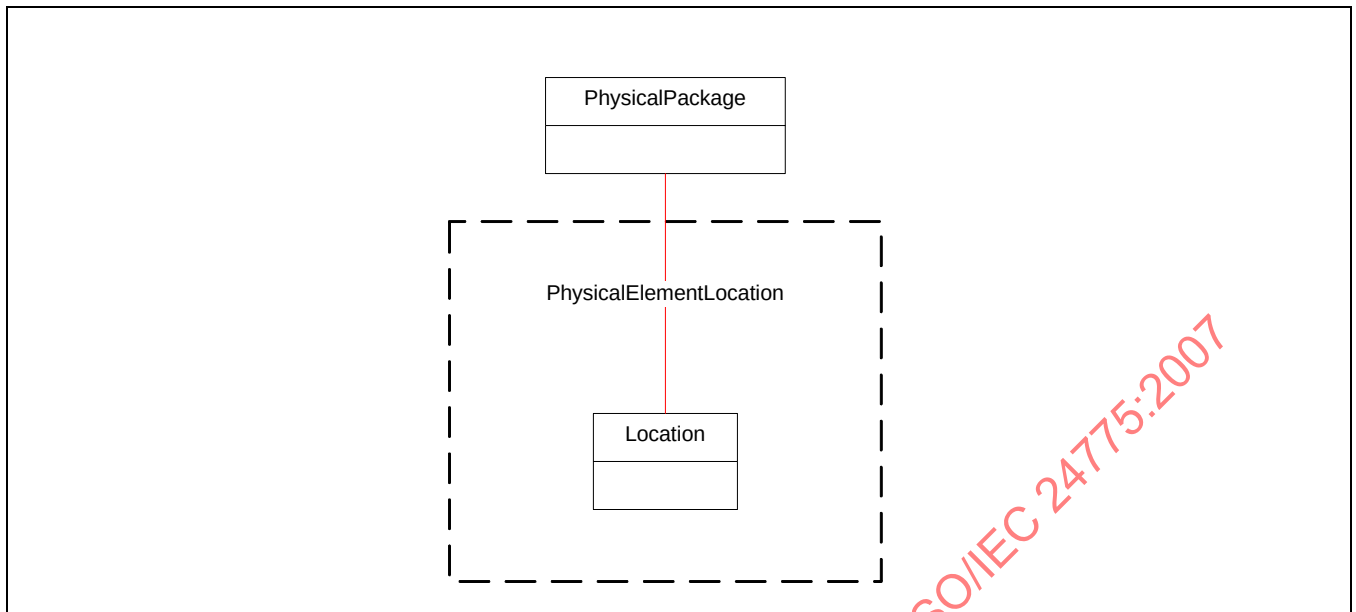
Figure 23 - Location Instance
