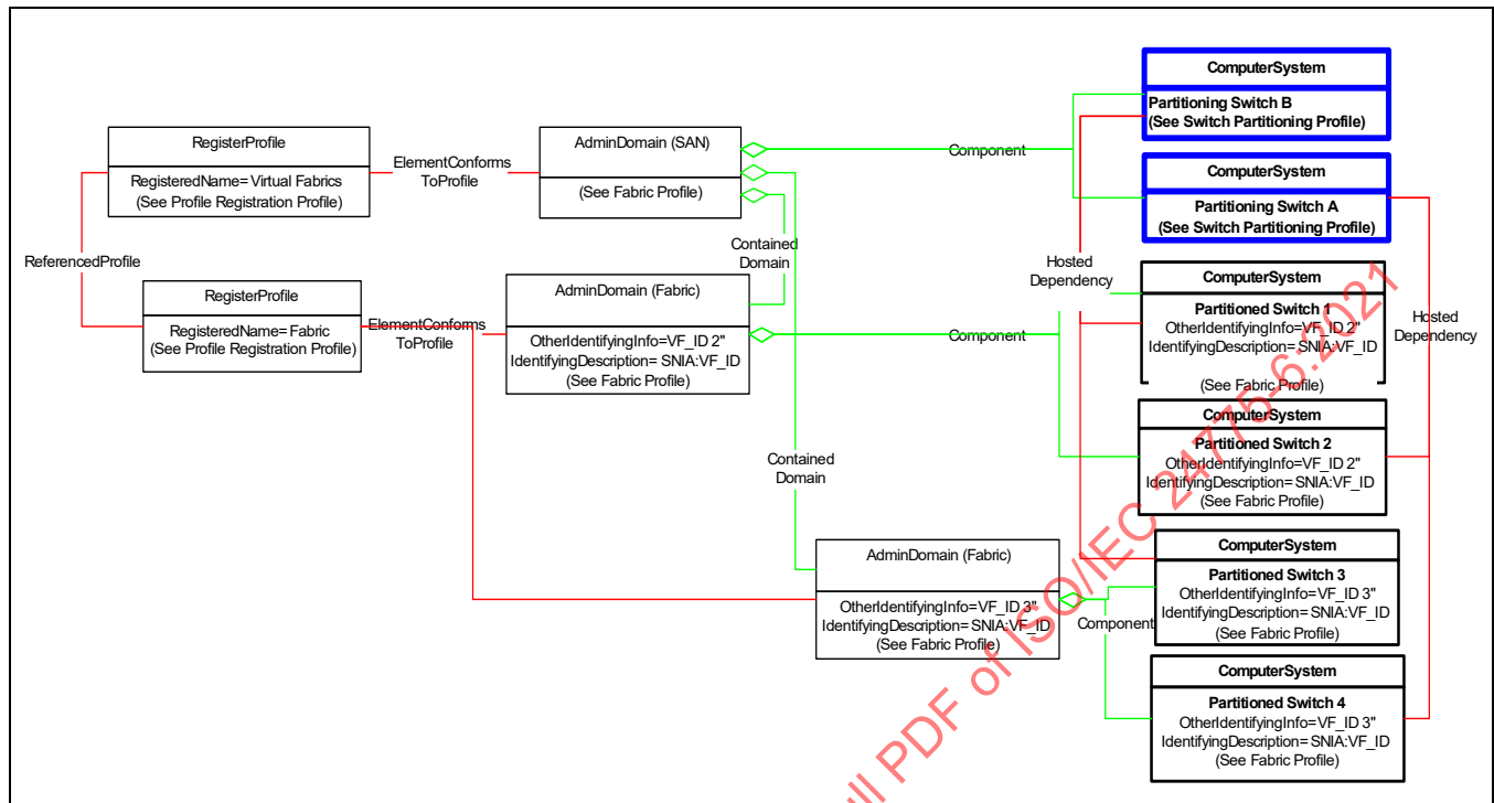
Figure 17 - RegisteredProfile, AdminDomain, and ComputerSystem Relationships
