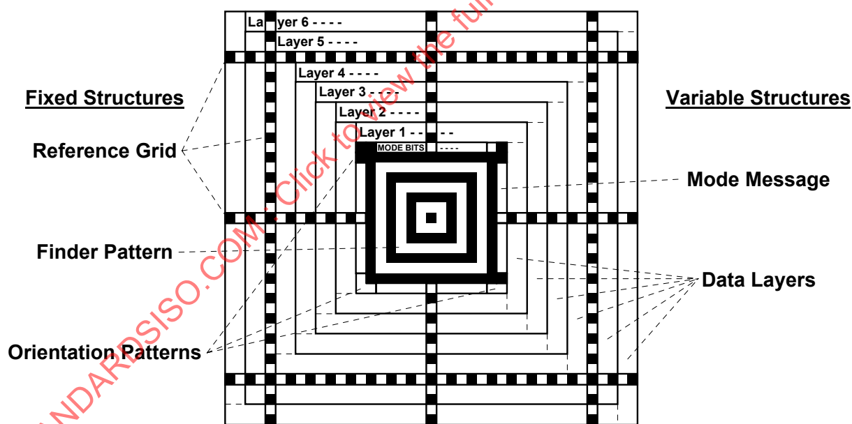
Figure 3 — Structure of a “full-range” Aztec Code symbol
