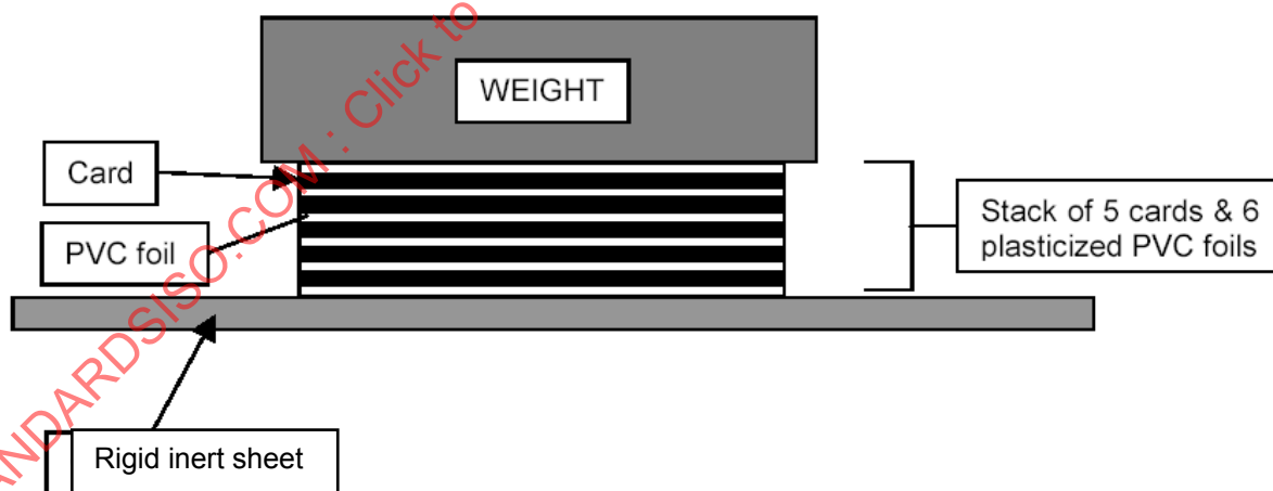
Figure 4 — Cards stacked for loading into the environmental chamber
