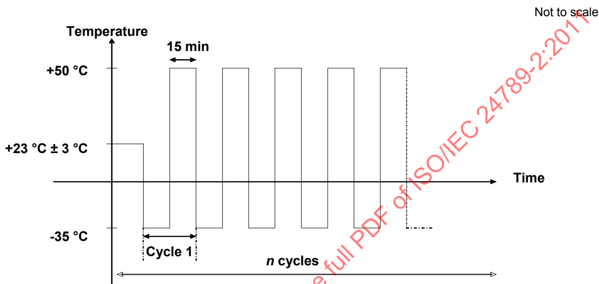
Figure 7 — Temperature shock cycles
