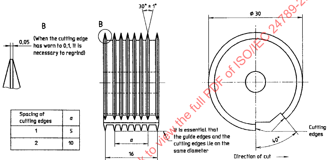
Figure 9 — Multi-blade cutting tool
