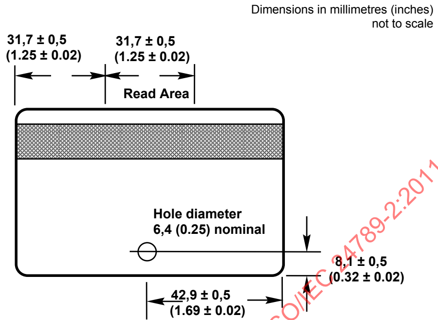
Figure 2 — Magnetic stripe read area and hole location
