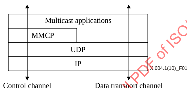
Figure 1 – Protocol model
