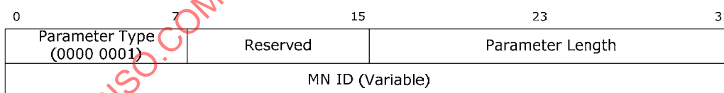
Figure 11 – Parameter of MN identifier
