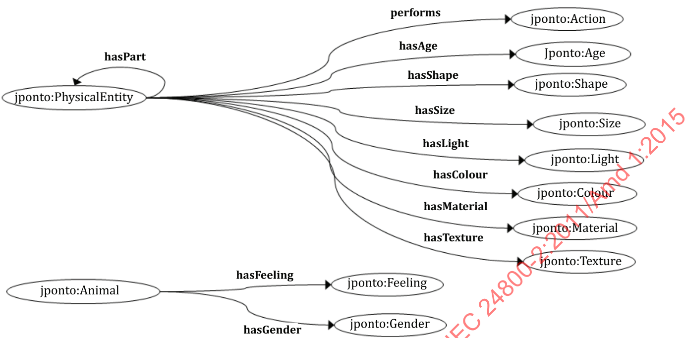
Figure 8 — Specific properties of JPonto-visual (arrows show the domain and range of the property)
