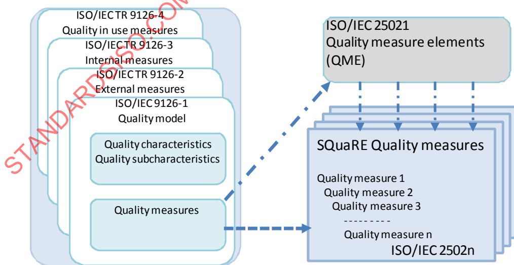
Figure 3 — The relationship of ISO/IEC 25021 as a link between the 9126 series and the SQuaRE series of standard
