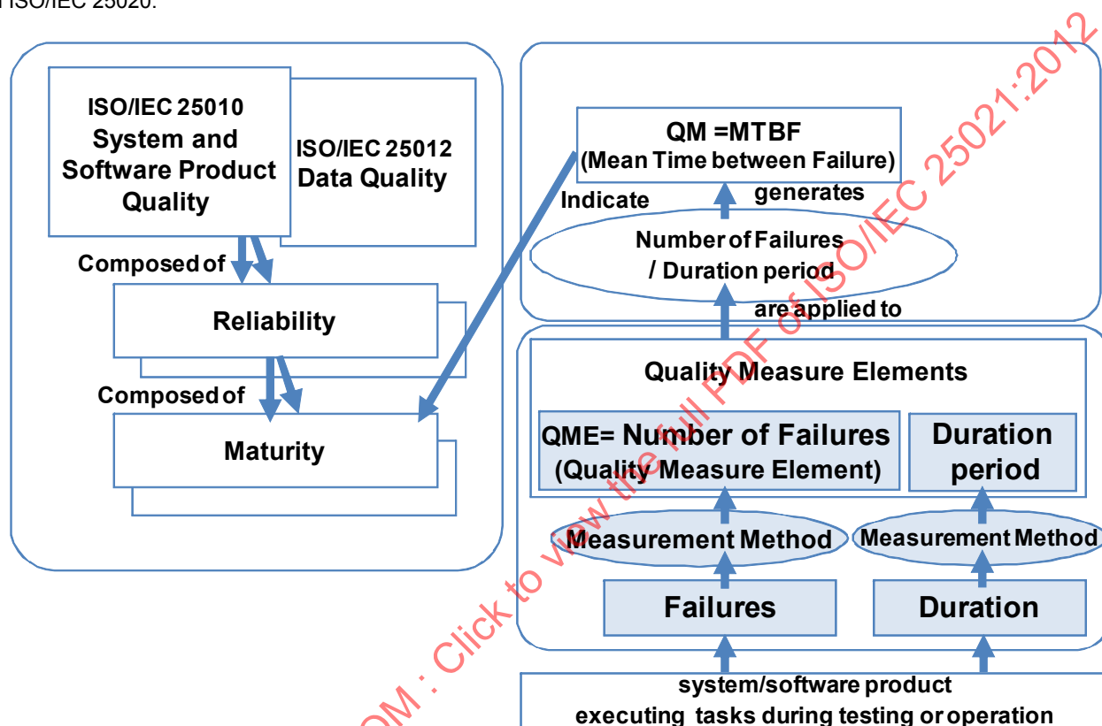
Figure 6 — An Example of Relationship among property to quantify, measurement method, QME and QM
