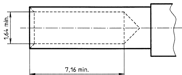
Figure 5 — Female contact
