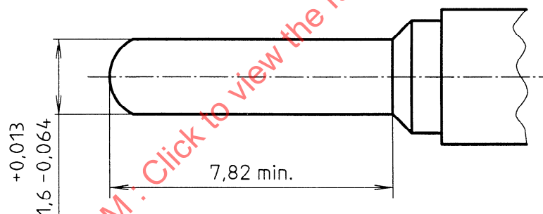
Figure 4 — Male contact
