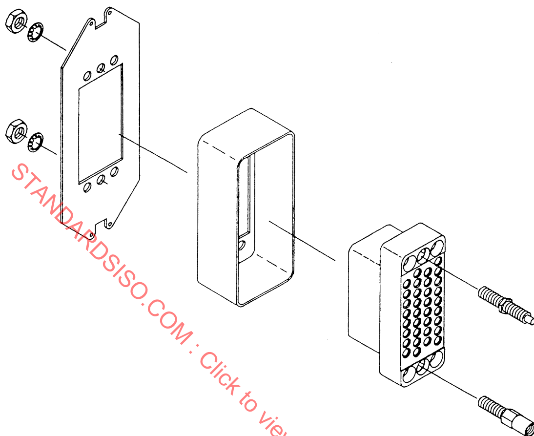
Figure 8 — DCE connector mounting illustration
