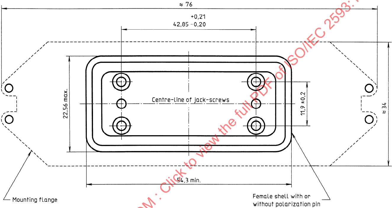
Figure 2 — DCE connector
