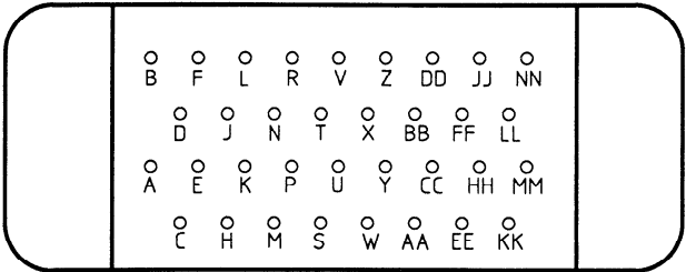
DTE contact arrangement viewed from connector front (DTE side)
