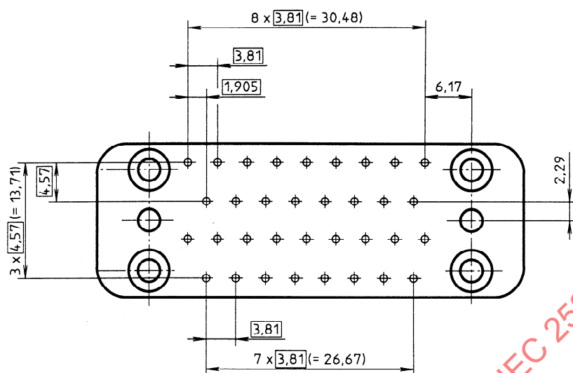
Figure 3 — Contact spacing dimensions
