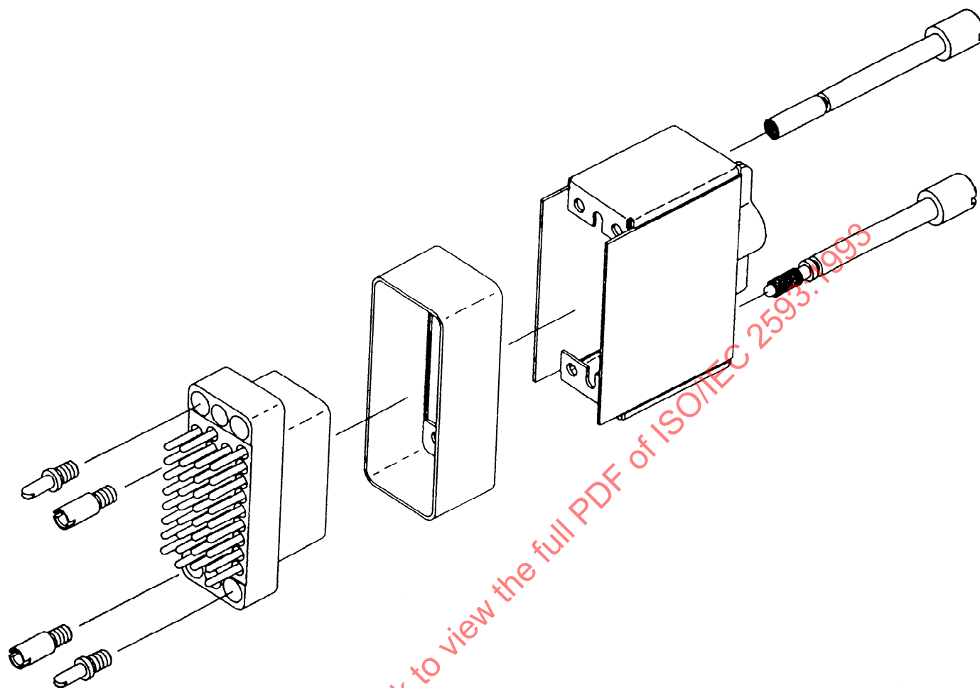
Figure 9 — DTE connector mounting illustration
