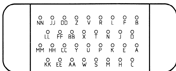
DTE contact arrangement viewed from connector front (DCE side)
