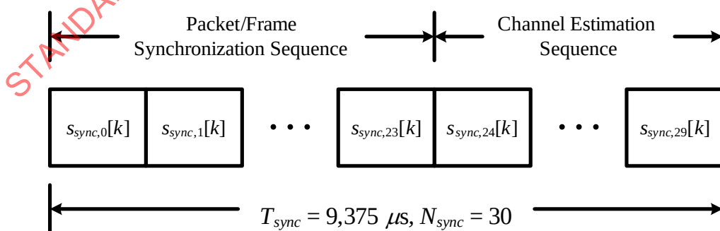
Figure 7 - Block diagram of the Standard PLCP preamble
