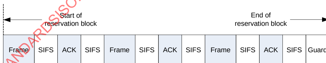
Figure 107 - SIFS and Guard Time in a DRP reservation block - Imm-ACK
