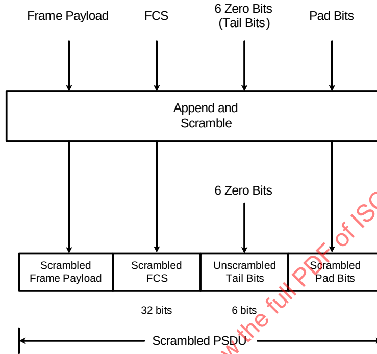
Figure 16 - Block diagram of PSDU construction
