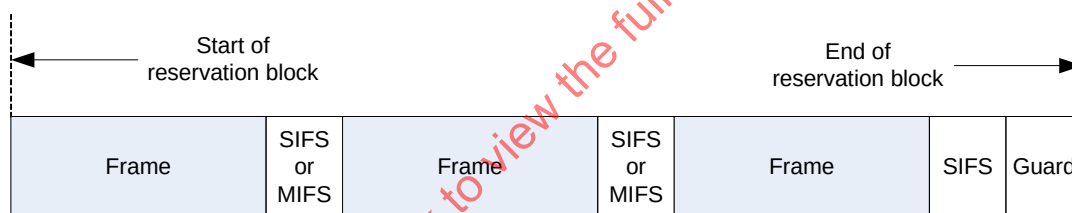
Figure 106 - SIFS and guard time in a DRP reservation block - No-ACK
