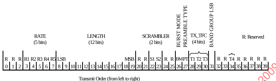
Figure 13 - PHY Header bit assignment
