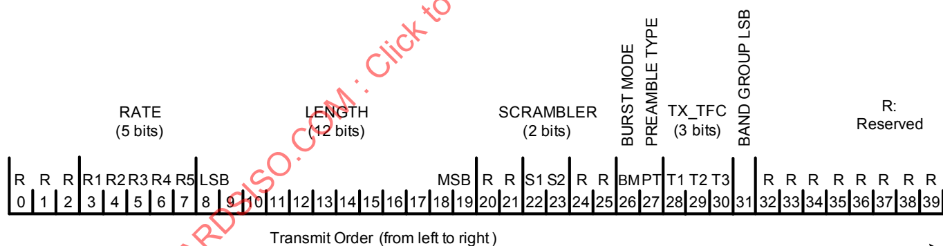
Figure 8 — PLCP Header Format
