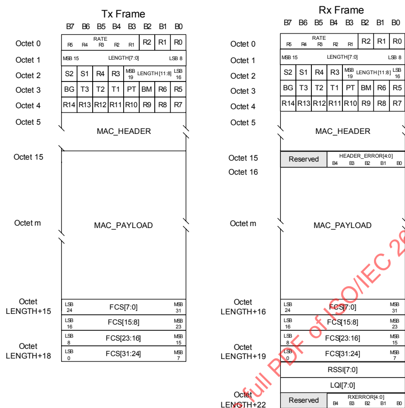
Figure 7 — Frame Structures for Transmit &amp; Receive States
