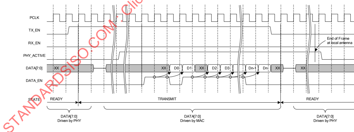
Figure 19 — Single Frame Transmit Timing
