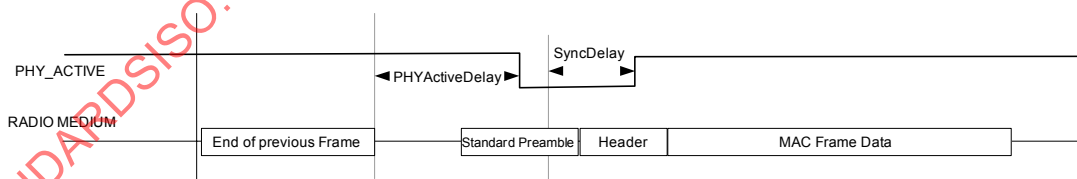
Figure 15 — PHYActiveDelay Timing
