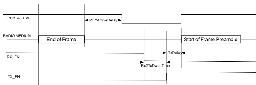
Figure 16 — Rx-Tx Turnaround Time
