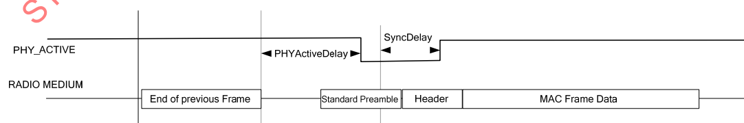
Figure 15 – PHYActiveDelay Timing
