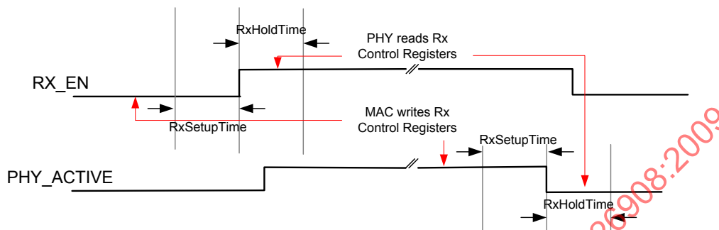
Figure 6 – Receive Control Register Setup & Hold
