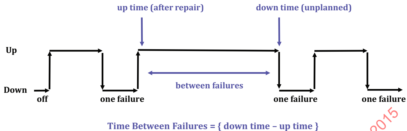
Figure 5 — Quantification of reliability
