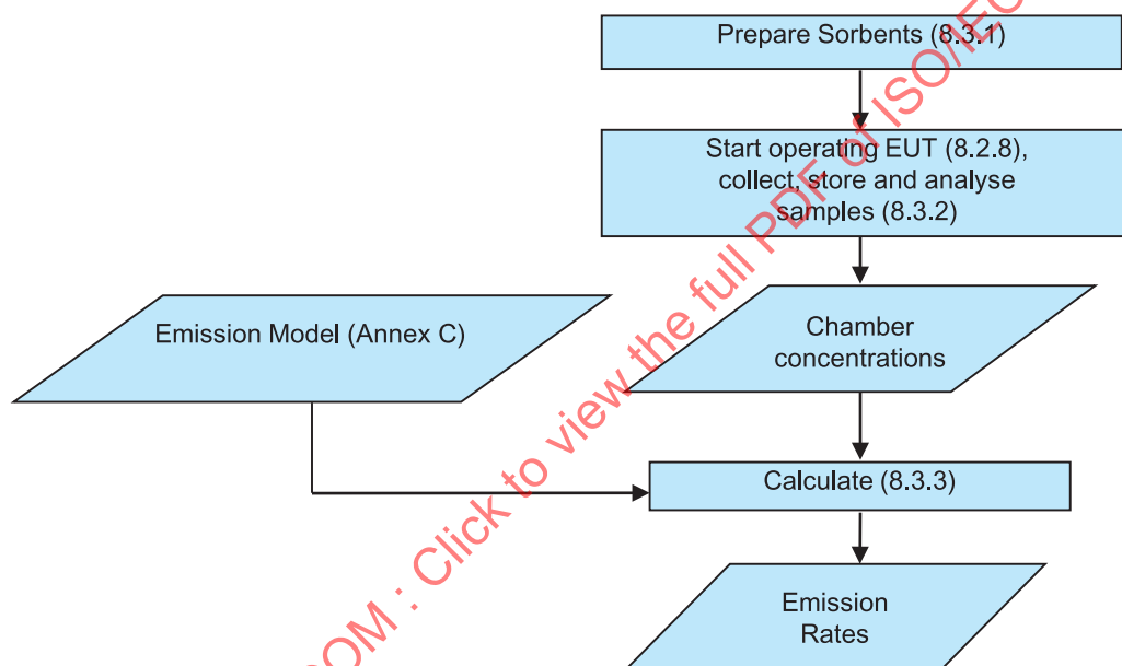
Figure 2 – Determination method for VOC, carbonyl compounds
