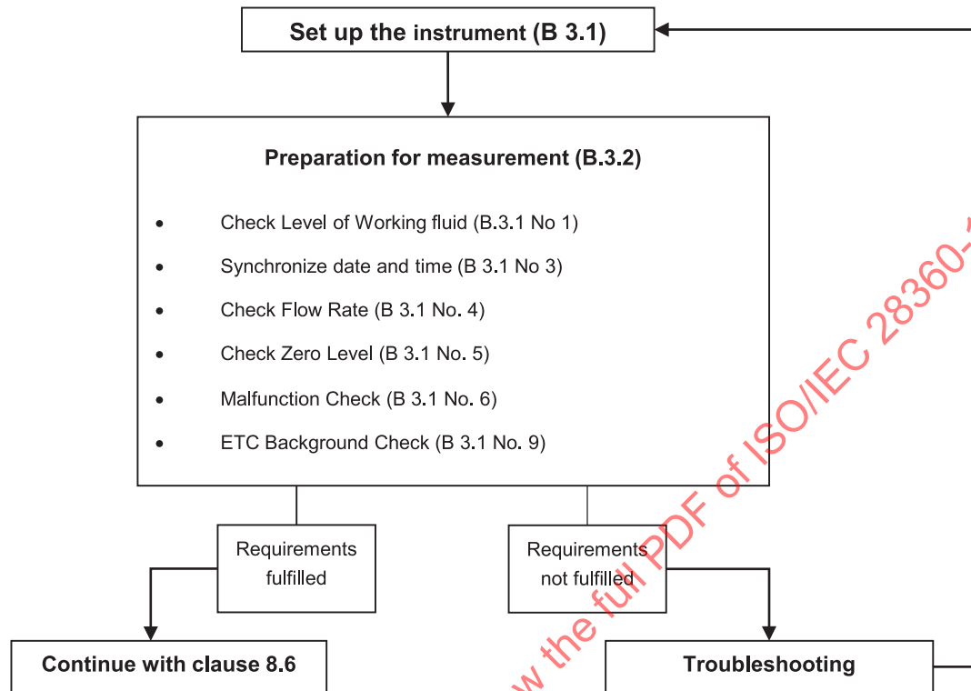
Figure B.2 — Preparation scheme for CPC
