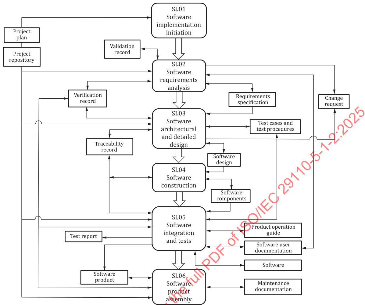
Figure 4 — Software implementation process
