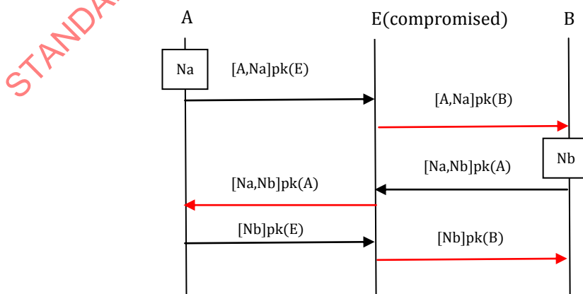
Figure B.1 — Man-in-the-middle-attack (G. Lowe 1995)
