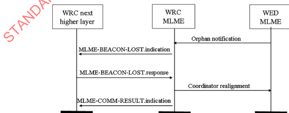
Figure 7 – Beacon lost (orphan notification) message sequence chart
