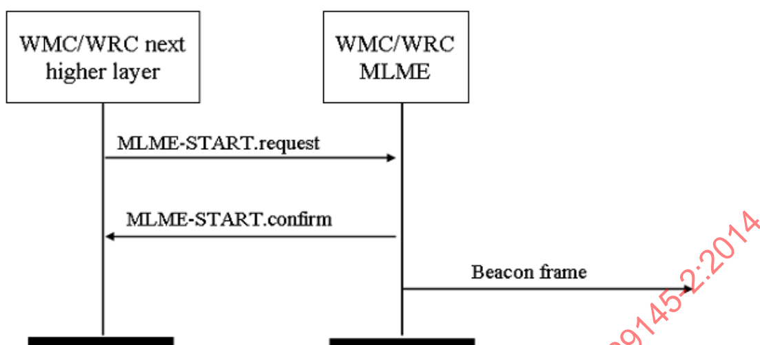
Figure 8 – Message sequence chart for updating the superframe configuration
