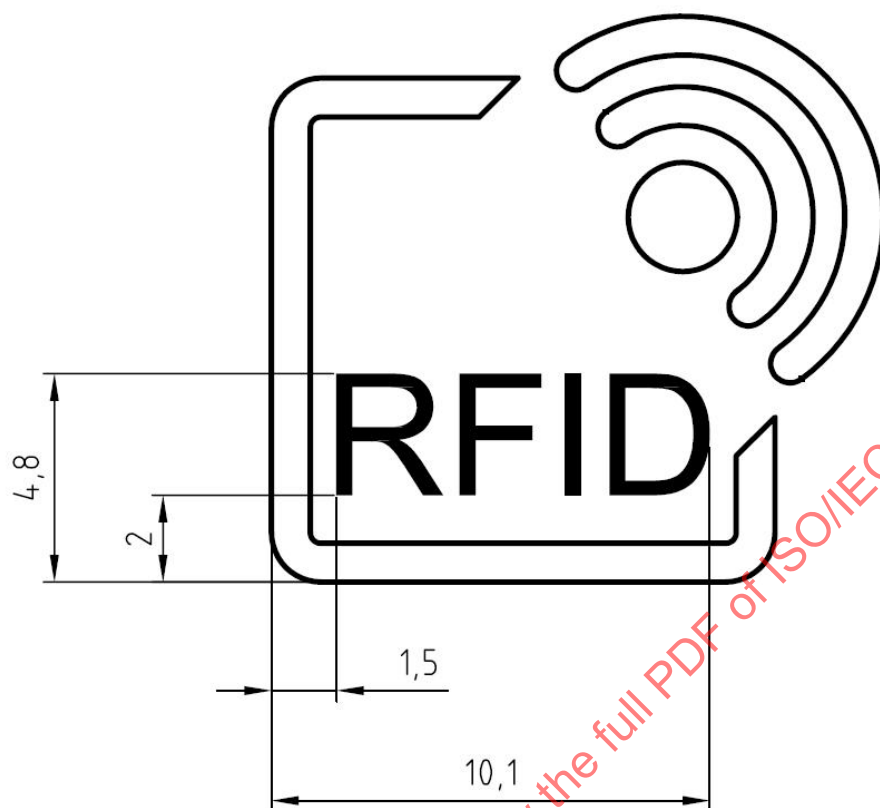
Figure B.2 — General purpose RFID Emblem
