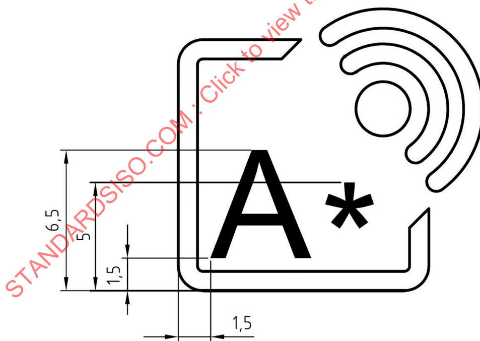
Figure B.5 — Example of RFID Emblem with interrogator code of ISO/IEC 18000-7 compatible interrogator
