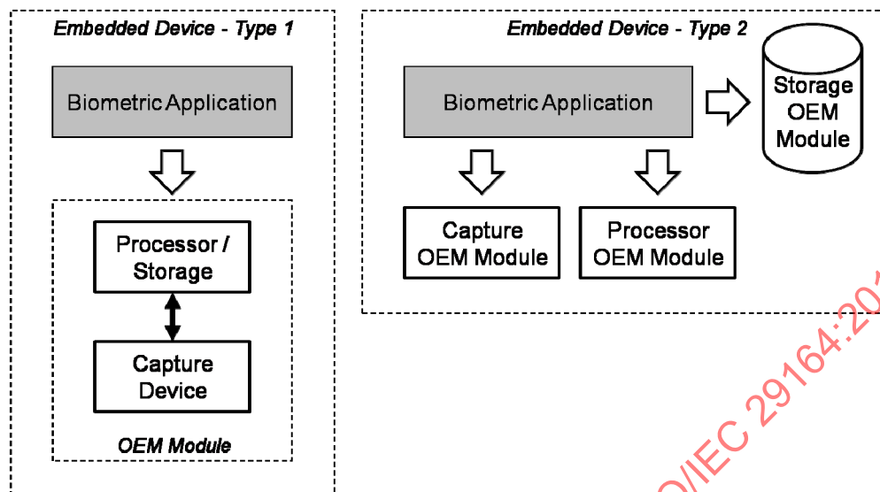
Figure 2 — Different ways to implement OEM biometric modules
