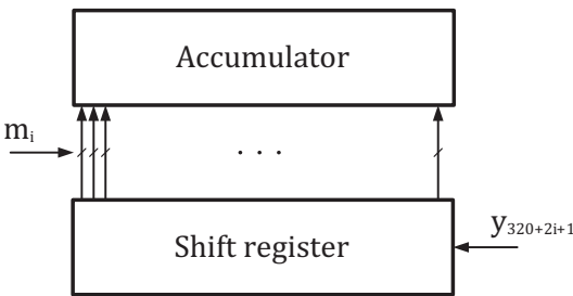
Figure C.3 — MAC32 Generator
