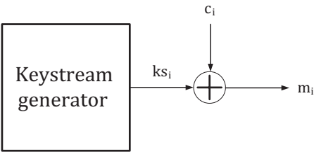
Figure C.5 — Decryption Operation
