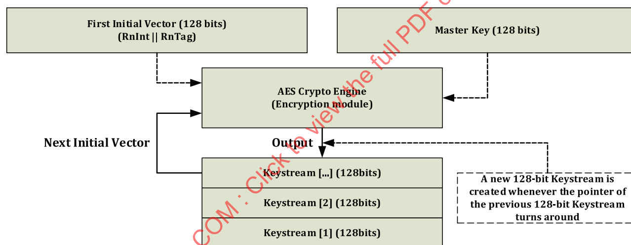
Figure 9 — Keystream Generation
