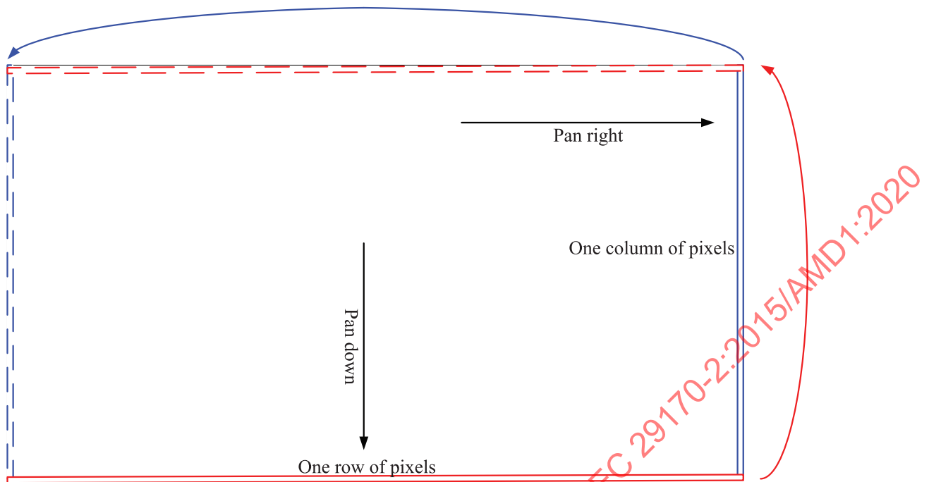
Figure C.5 — Panning image sequence preparation by circular shift
