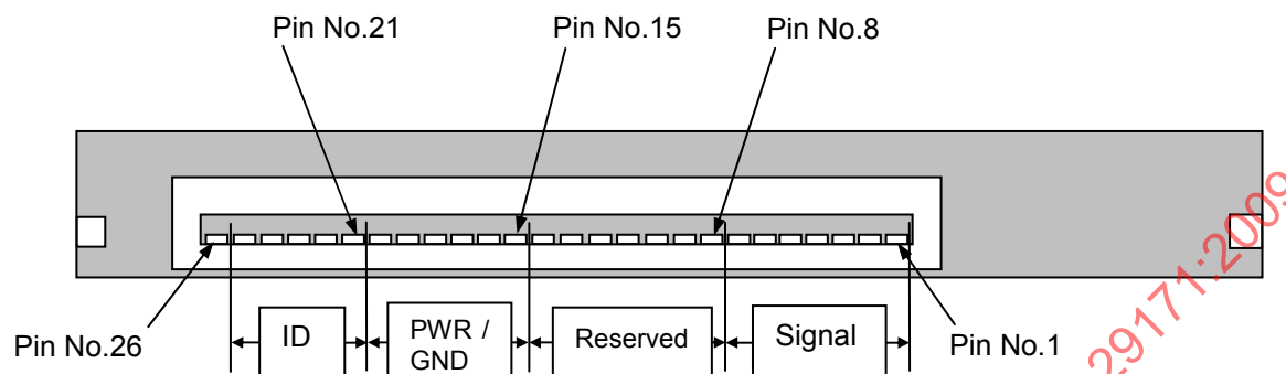
Figure 13 — Pin configuration of iVDR cartridge plug connector
