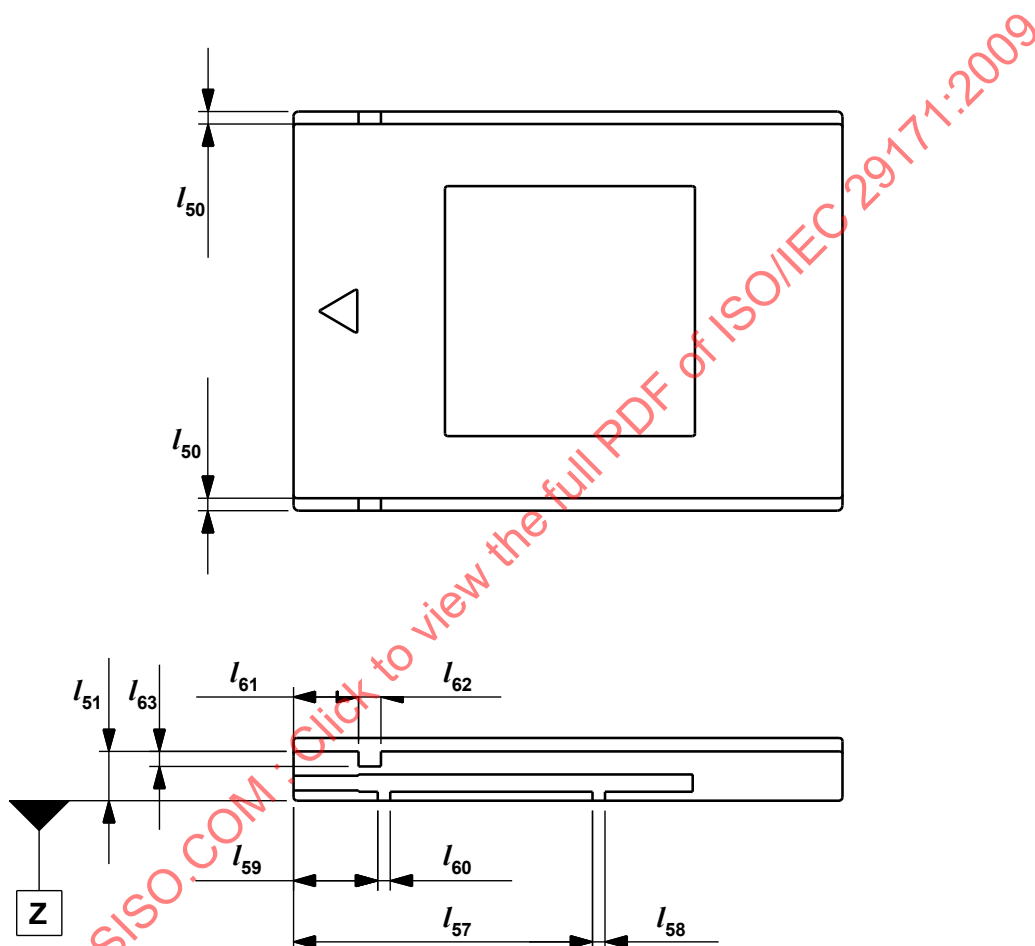
Figure 7 — Gaps for locking system
