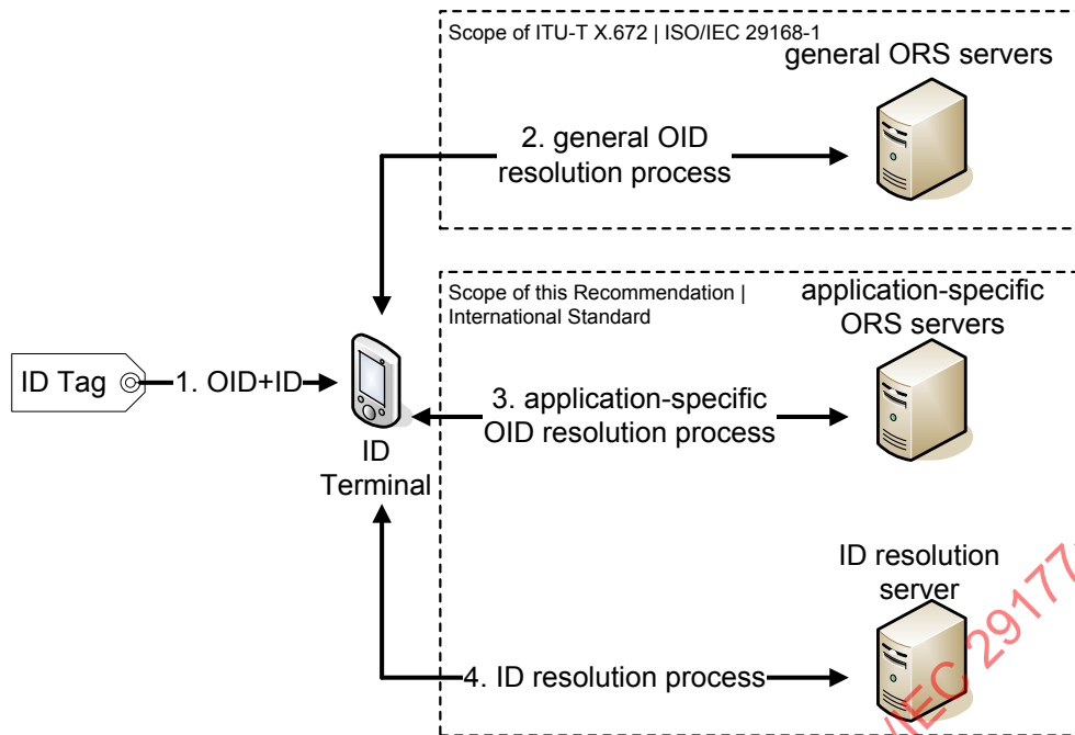
Figure 1 – Overall procedure of ID resolution
