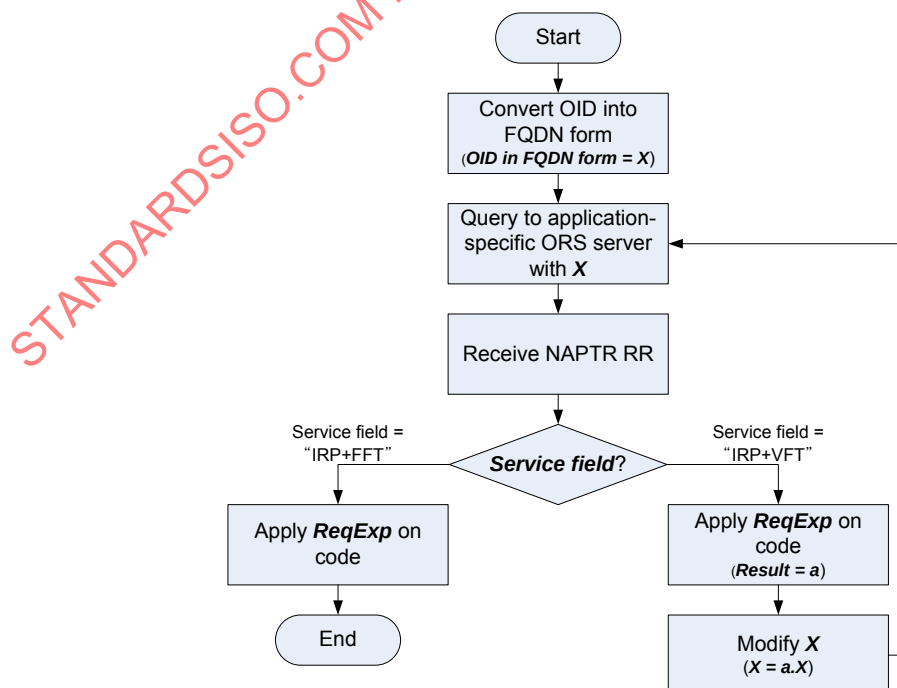
Figure 2 – Operation of application-specific OID resolution process
