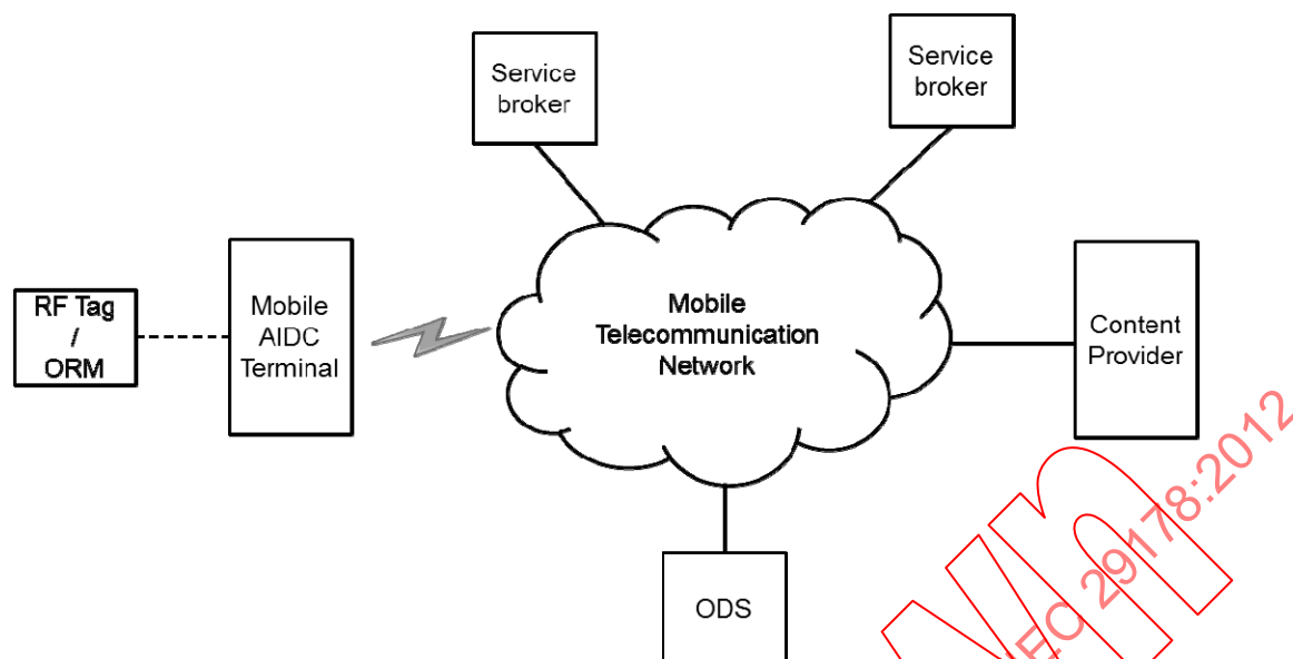
Figure 3 — Service broker-assisted architecture
